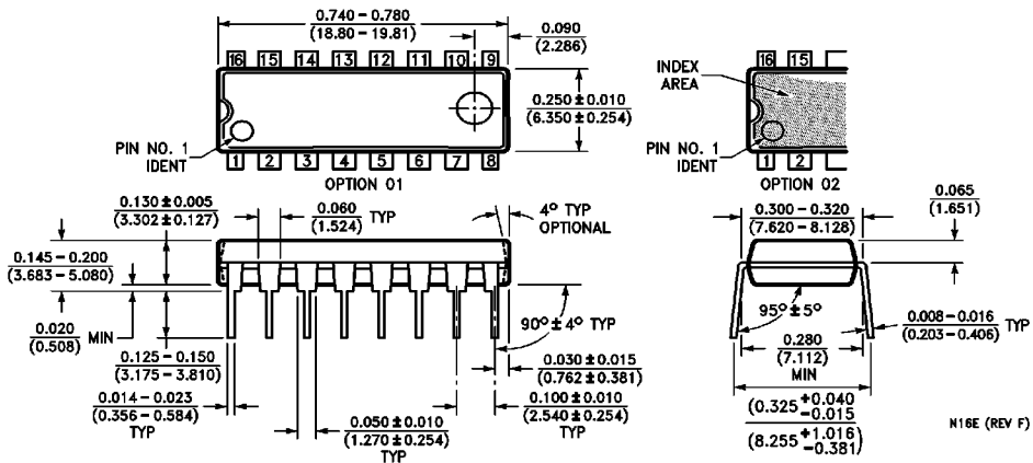
16-Lead (0.300" Wide) Molded Dual-In-Line Package (P) NS Package Number N16E
