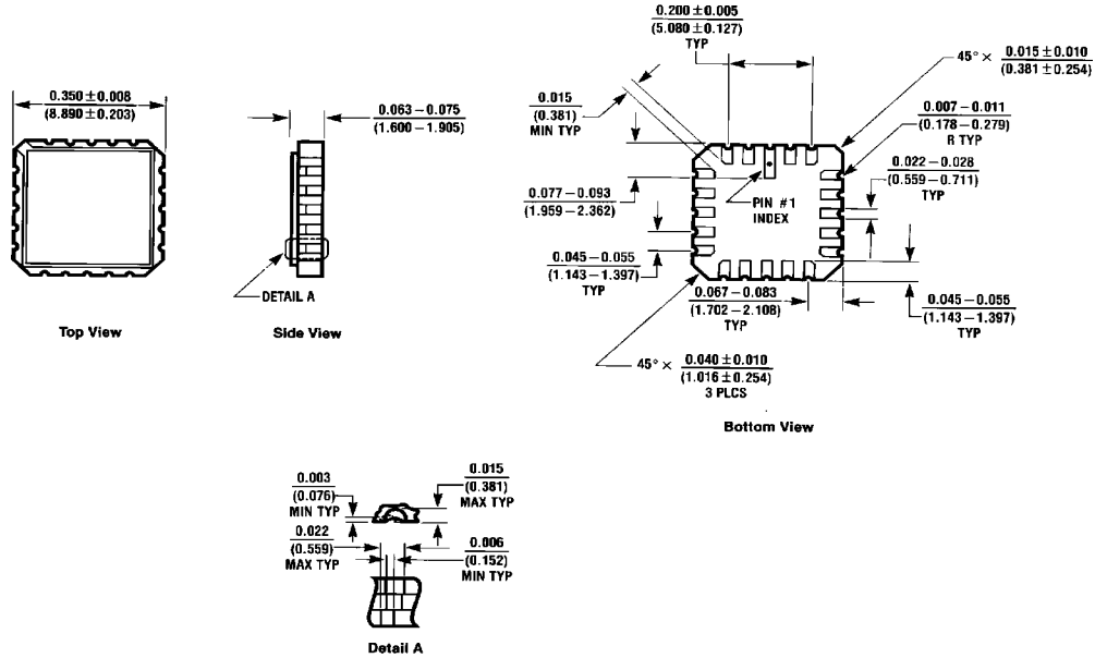
20-Lead Ceramic Leadless Chip Carrier (L) NS Package Number E20A
