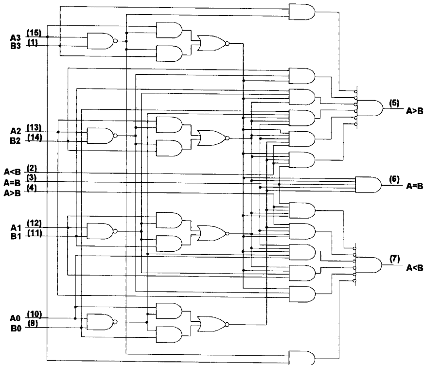
LOGIC DIAGRAM
