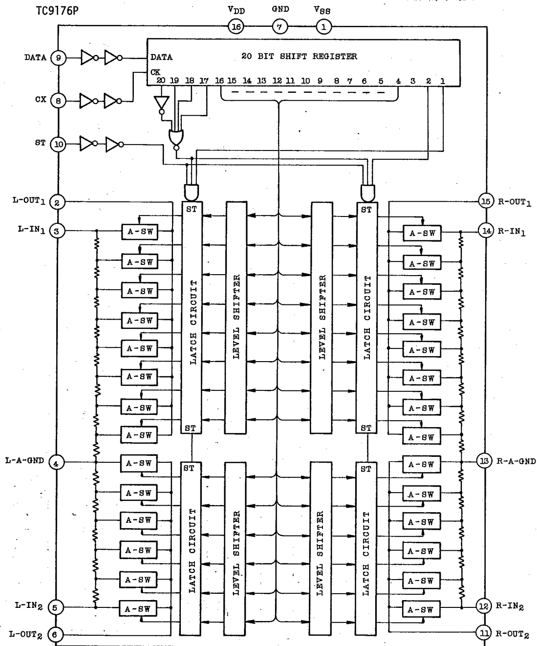
BLOCK DIAGRAM
