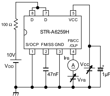
Measurement Circuit 5
