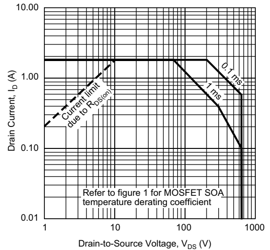
Figure 2 – MOSFET Safe Operating Area Drain Current versus Voltage
