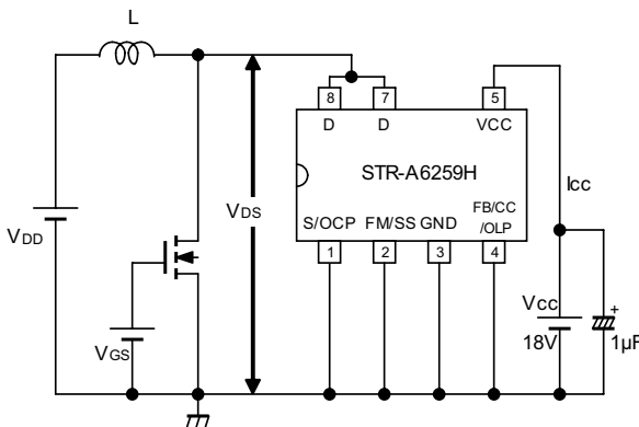
Measurement Circuit 7
