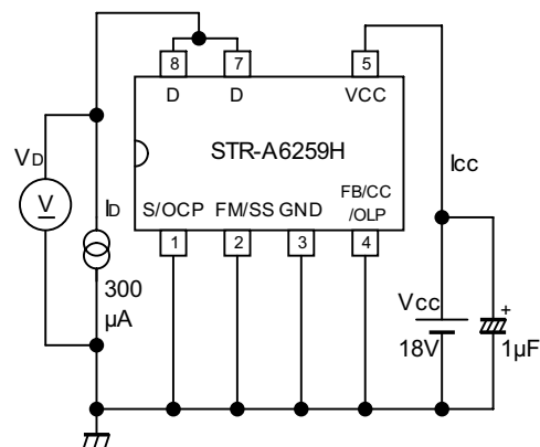
Measurement Circuit 7
