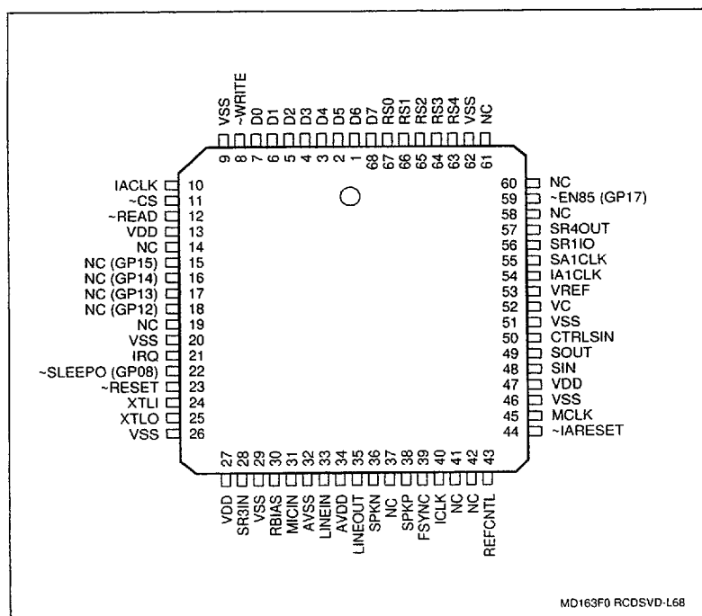
Figure 6. DSVD Coprocessor Pin Signals- 68-Pin PLCC
