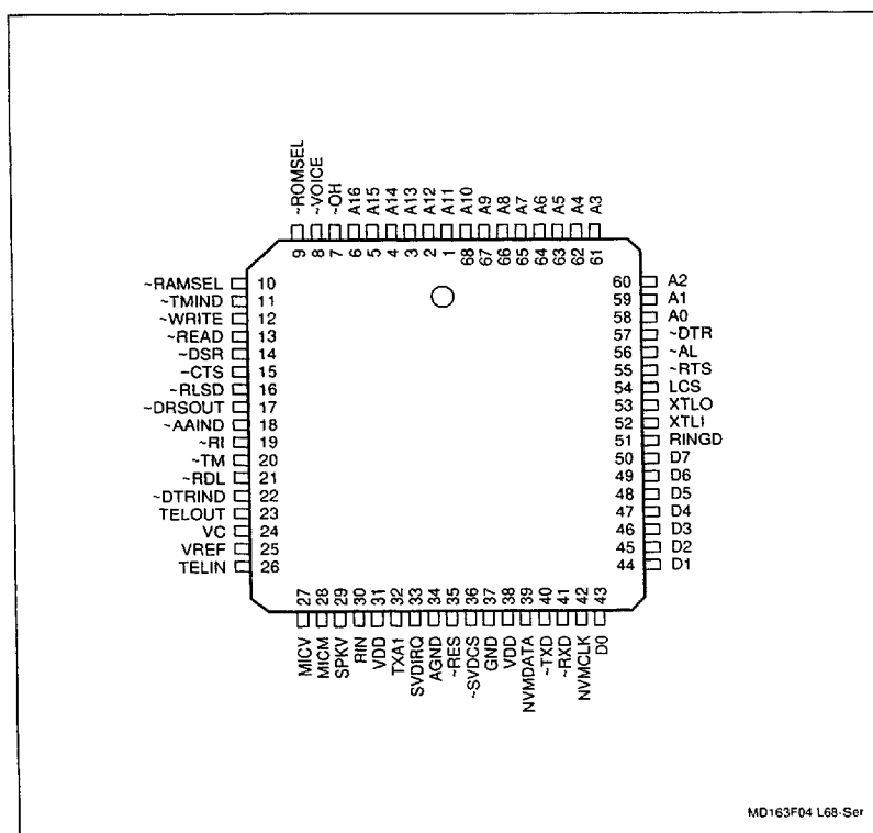
Figure 4. Modem Pin Signals - 68-Pin PLCC - Serial DTE Interface
