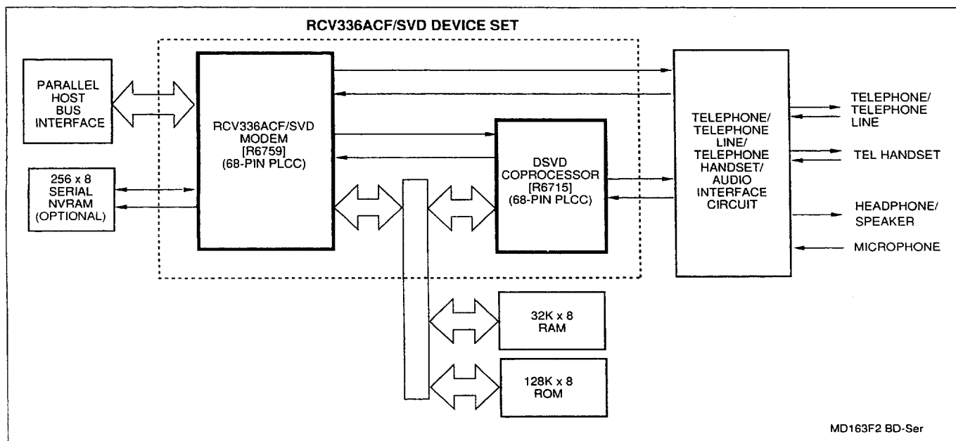
Figure 2. Block Diagram - Parallel Host Interface
