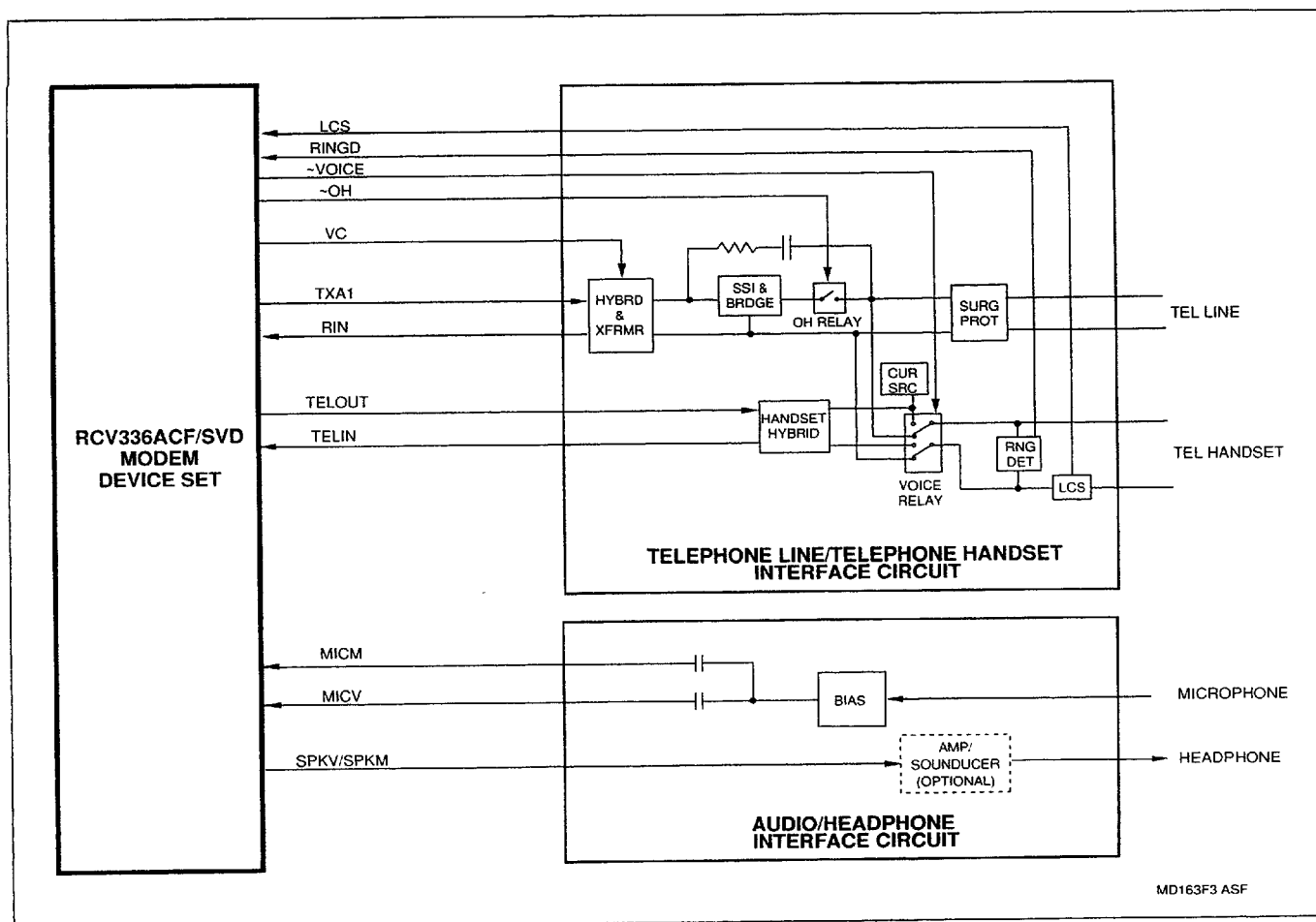
Figure 3. Typical Audio Signal Interface
