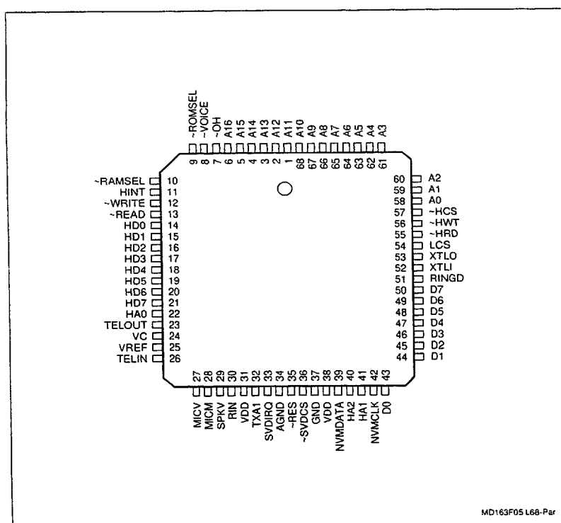
Figure 5. Modem Pin Signals- 68-Pin PLCC - Parallel Host Interface
