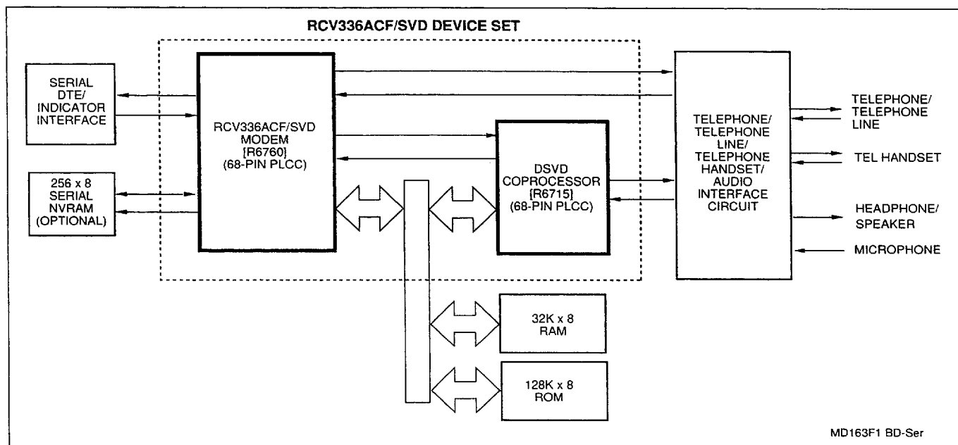
Figure 1. Block Diagram - Serial DTE Interface
