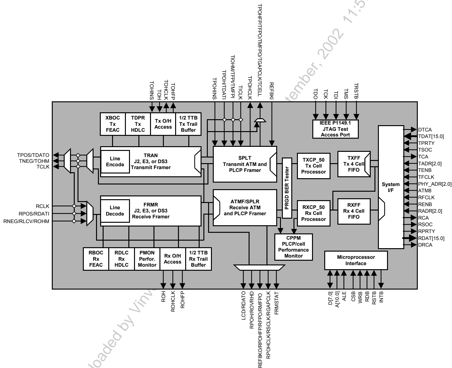
Figure 3 Block Diagram
