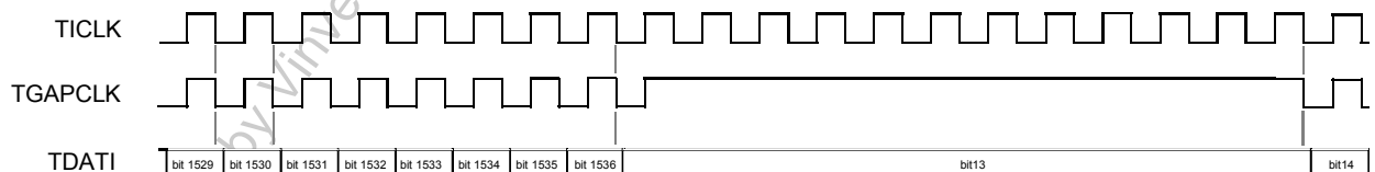
Figure 62 Framer Mode G.751 E3 Transmit Input Stream With TGAPCLK
