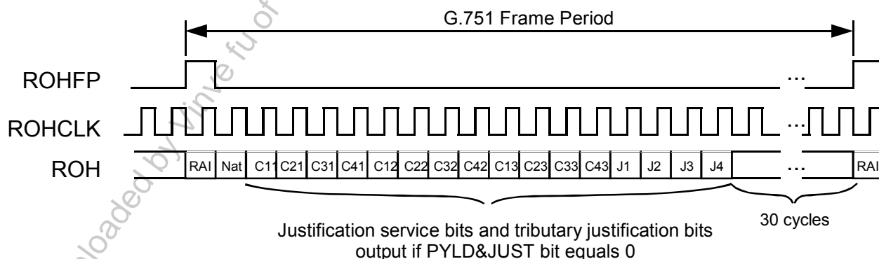
Figure 40 Receive G.751 E3 Overhead
