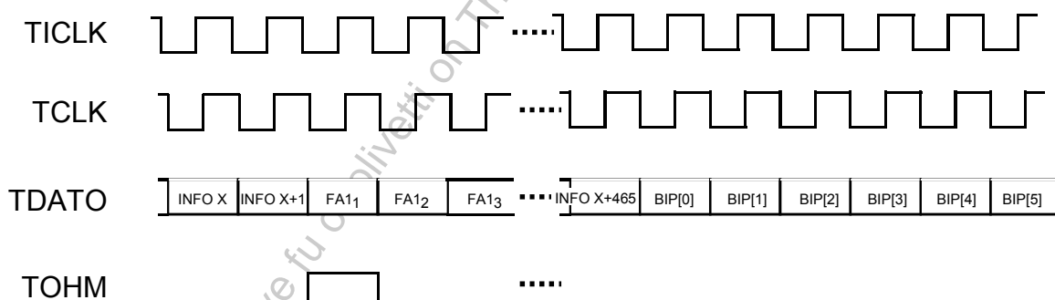
Figure 48 Transmit Unipolar E3 Stream
