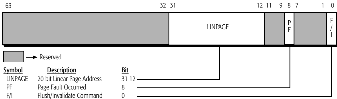
Figure 82. Page Flush/Invalidate Register (PFIR)—MSR C000_0088h
