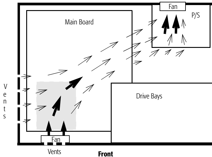
Figure 110. Airflow Path in a Dual-Fan System
