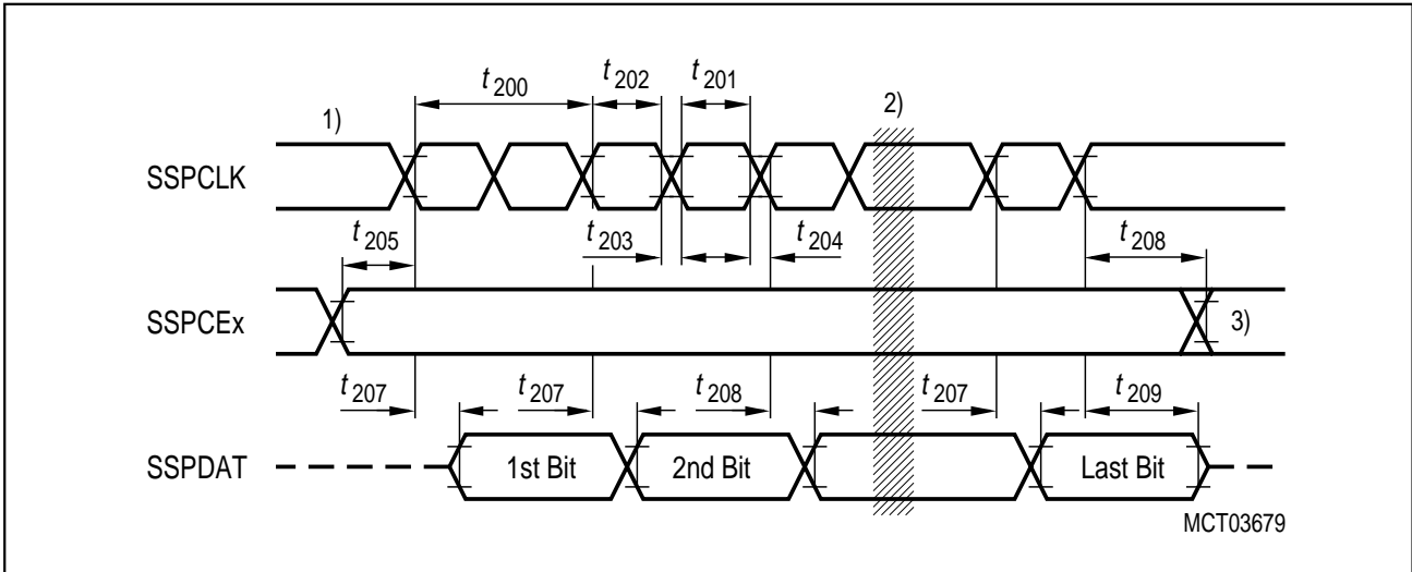
Figure 21 SSP Write Timing
