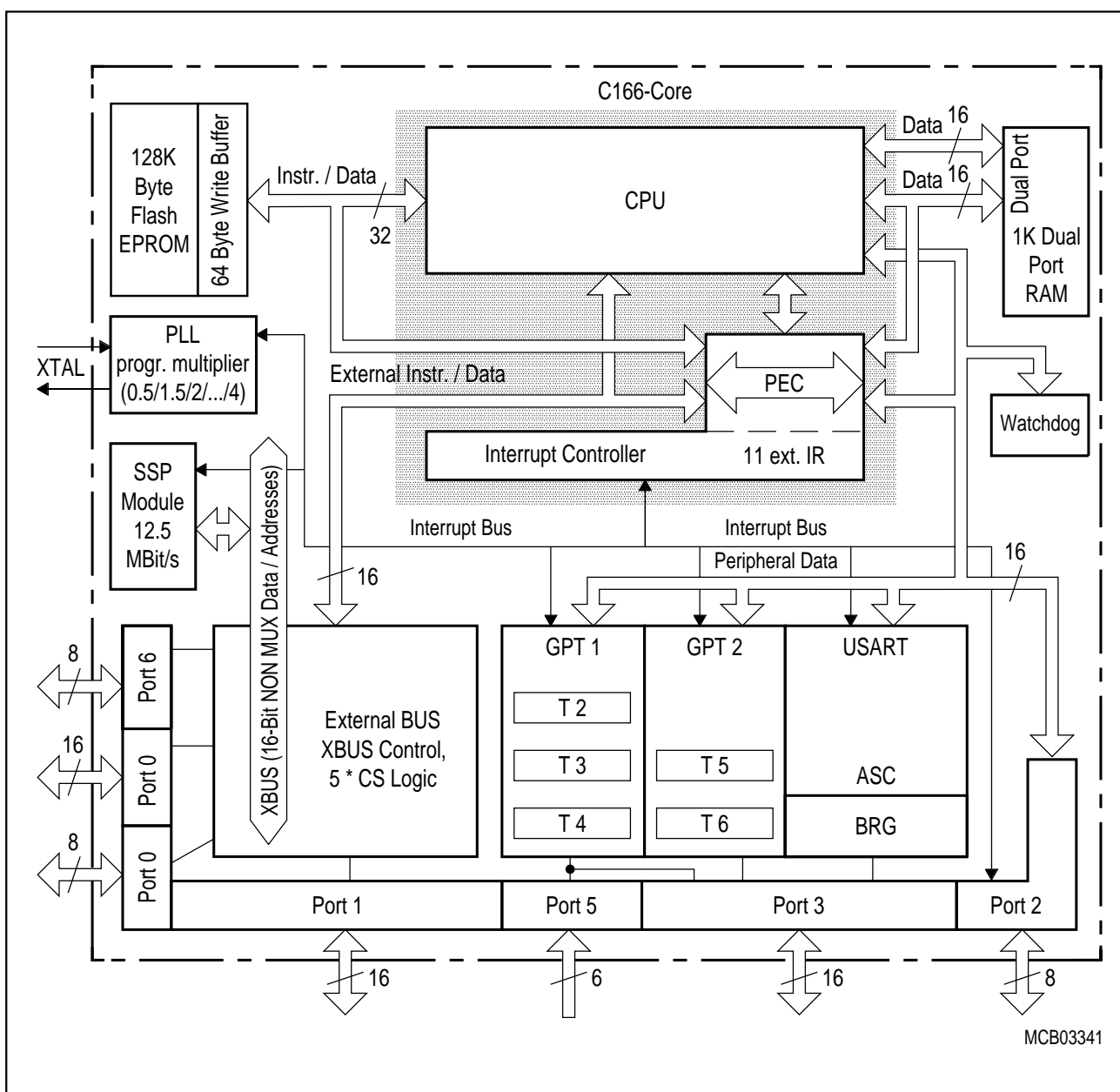
Figure 3 Block Diagram
