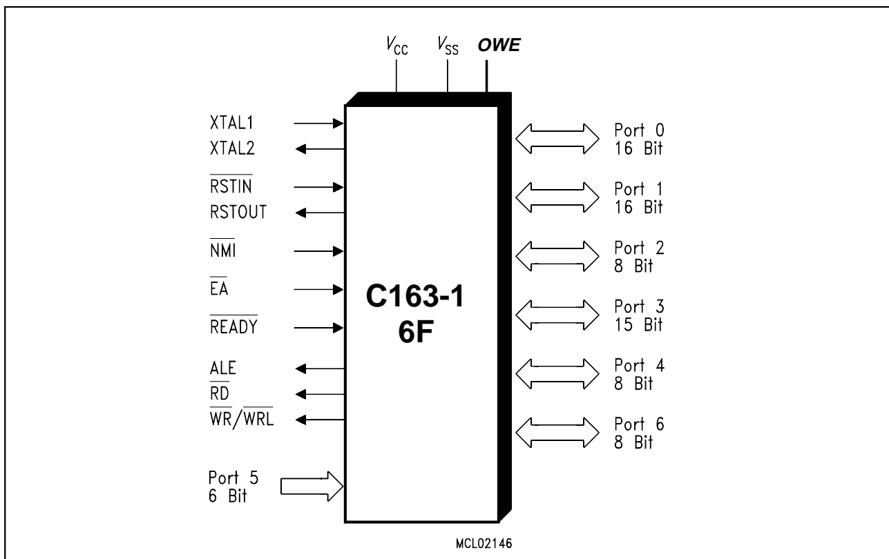
Figure 1 Logic Symbol
