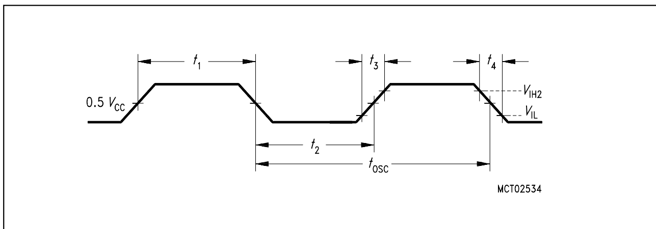
Figure 14 External Clock Drive XTAL1
