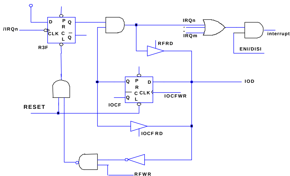
Fig. 9 Interrupt input circuit
