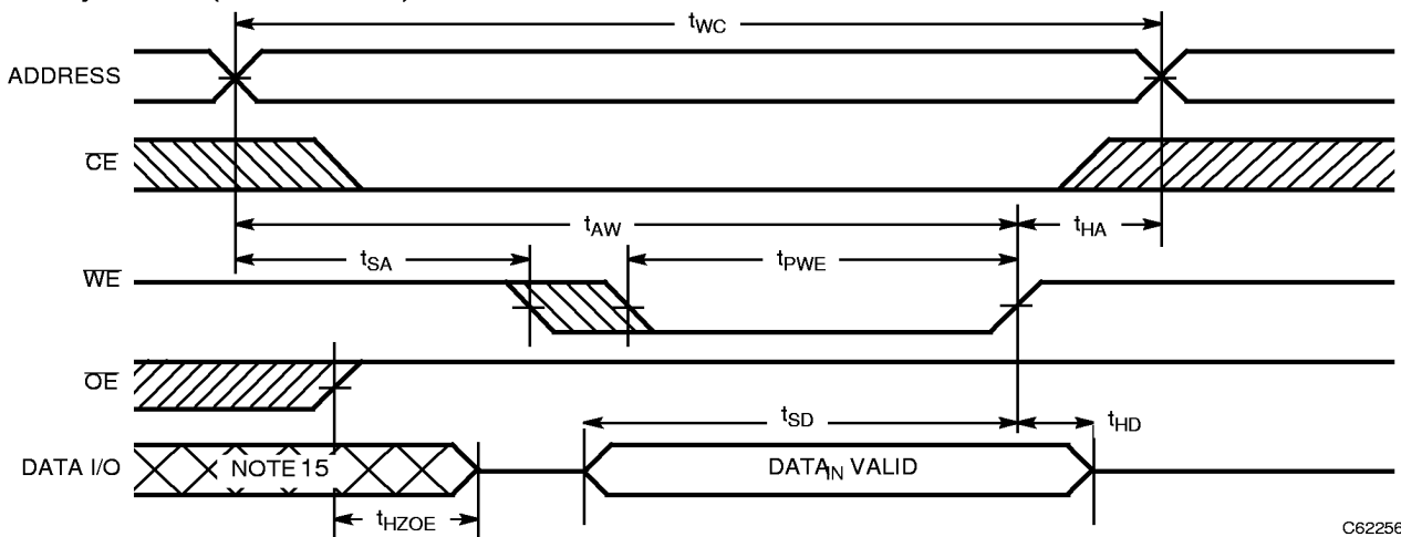
Write Cycle No. 1 (WE Controlled) [8,13,14]
