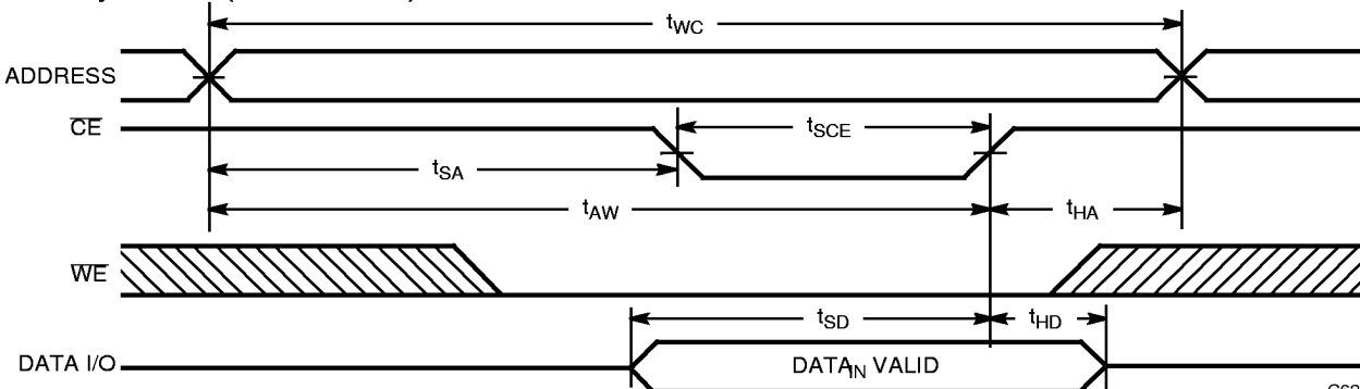
Write Cycle No. 2 (CE Controlled) [8,13,14]
