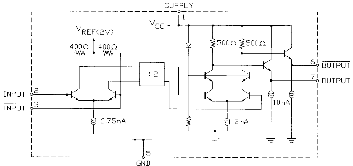
FIGURE 2. Block diagram.
