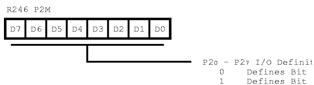
Figure 36. Port 2 Mode Register (F6 H : Write Only)
