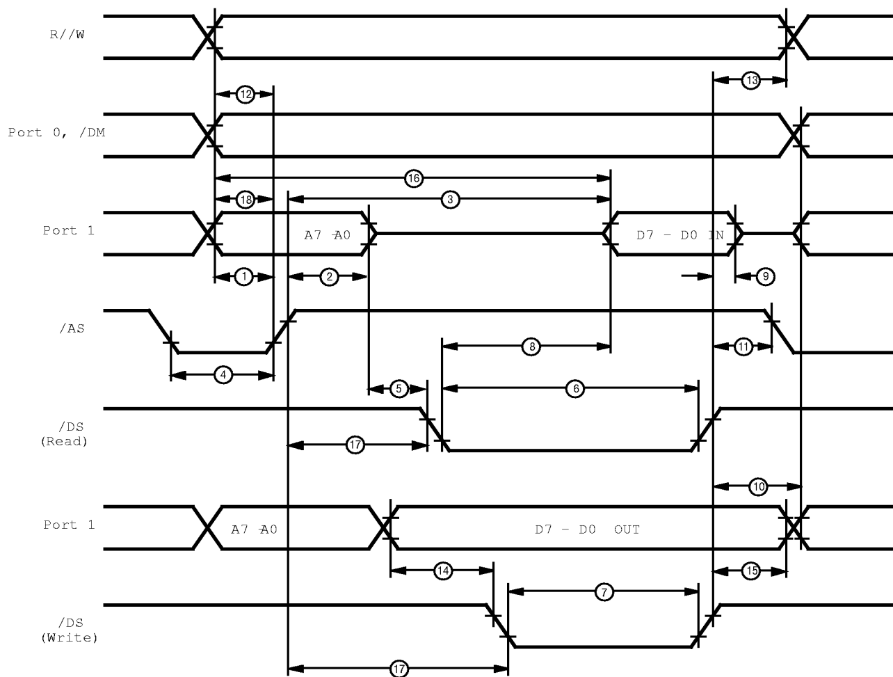
Figure 26. External I/O or Memory Read/Write
