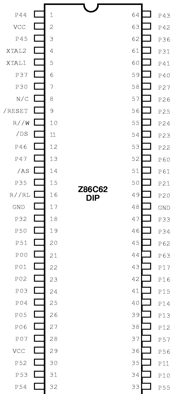
Figure 6. Z86C62 64-Pin DIP Pin Assignments
