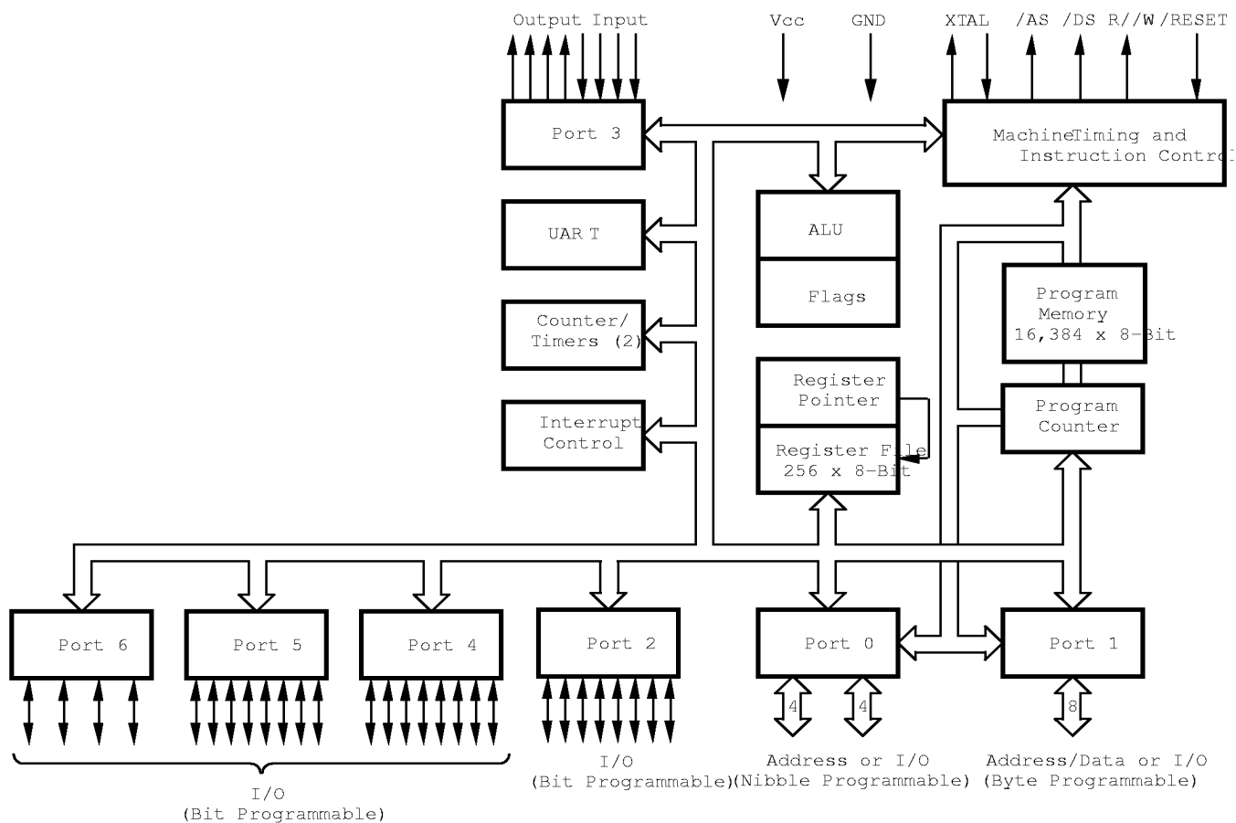
Figure 2. Z86C62 Functional Block Diagram
