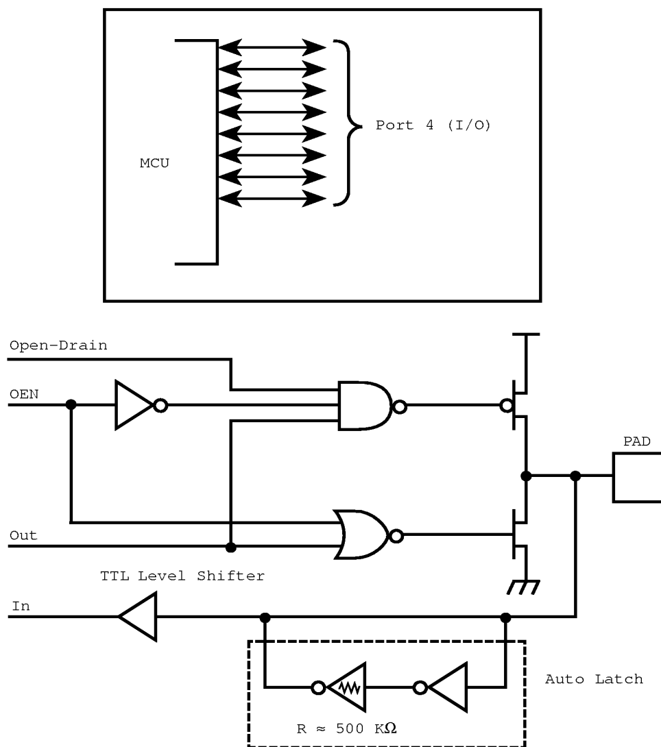
Figure 15. Port 4 Configuration
