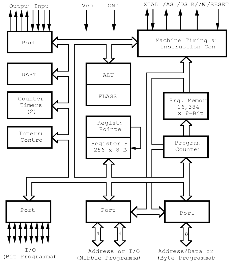
Figure 1. Z86C61 Functional Block Diagram
