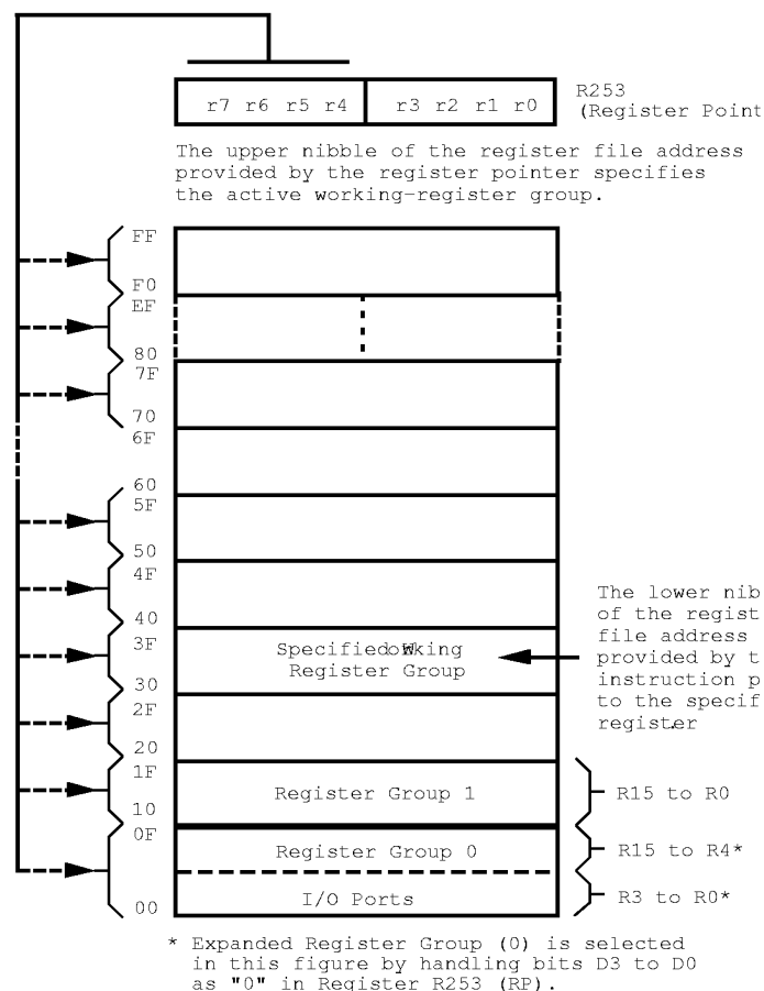
Figure 21. Register Pointer
