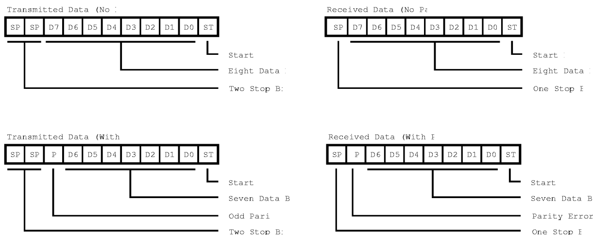
Figure 14. Serial Data Formats
