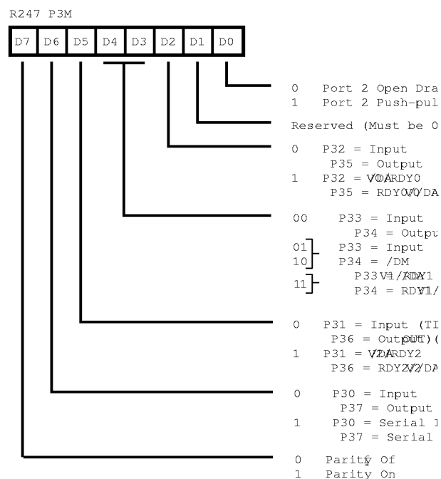
Figure 37. Port 3 Mode Register (F7 H : Write Only)
