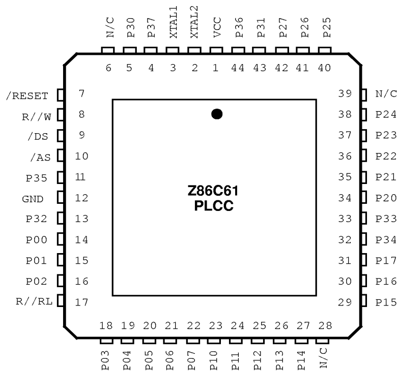
Figure 5. Z86C61 44-Pin PLCC Pin Assignments
