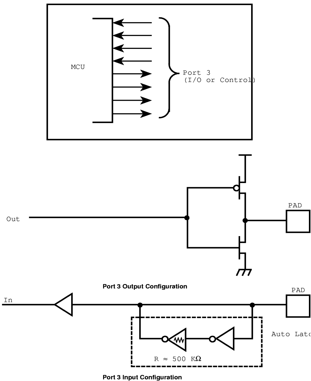
Figure 13. Port 3 Configuration
