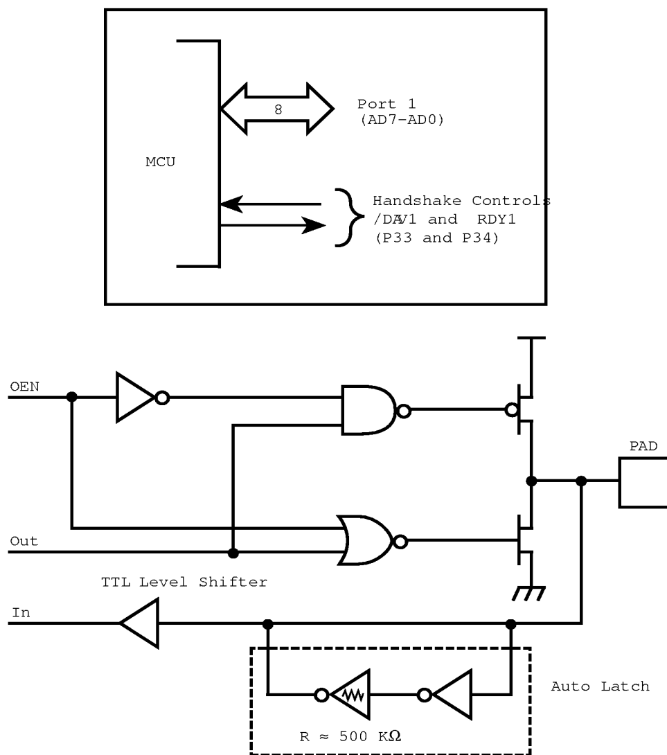
Figure 11. Port 1 Configuration
