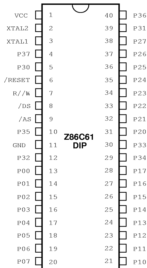
Figure 4. Z86C61 40-Pin DIP Pin Assignments
