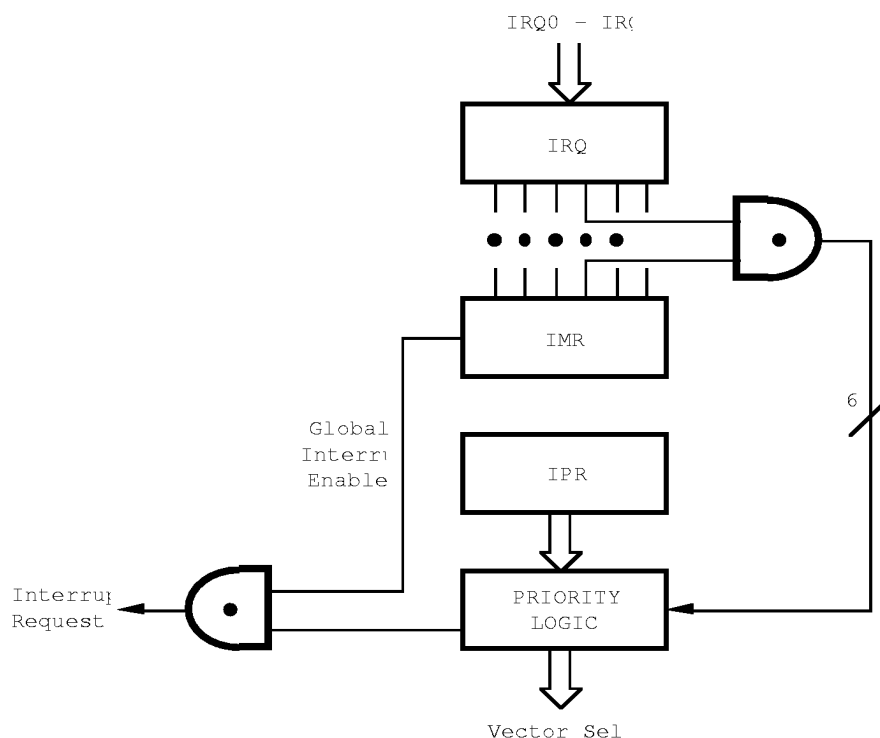
Figure 23. Interrupt Block Diagram
