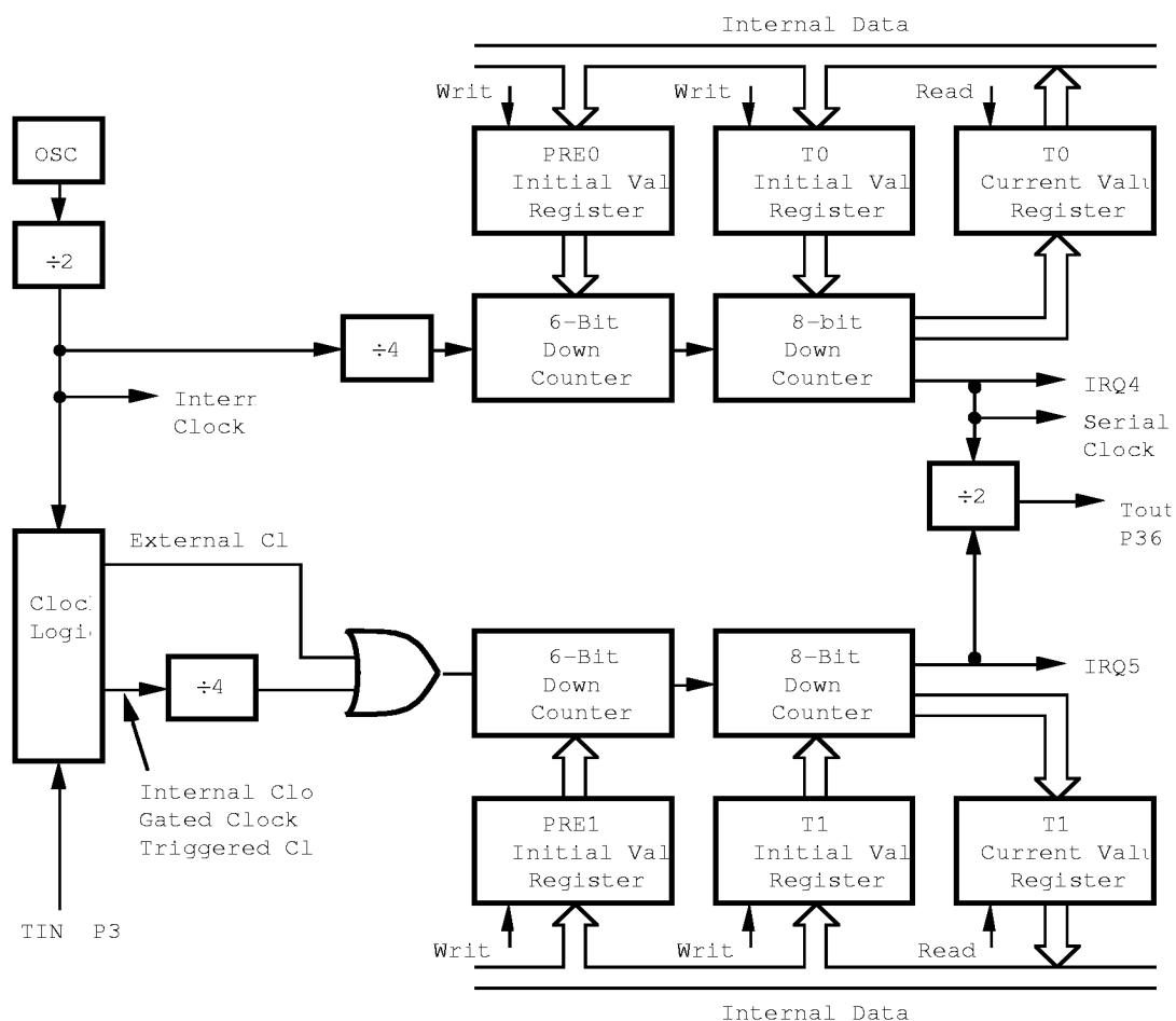
Figure 22. Counter/Timers Block Diagram
