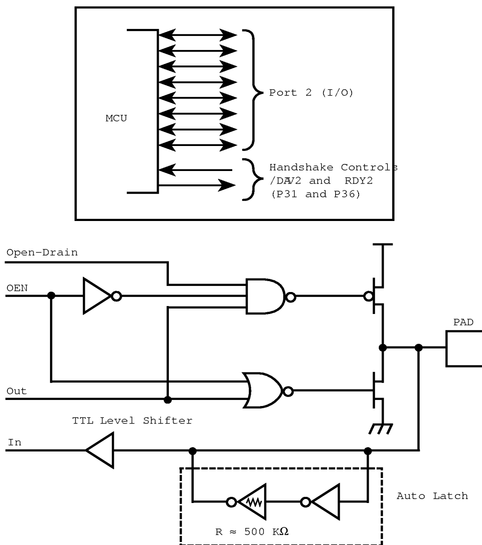
Figure 12. Port 2 Configuration
