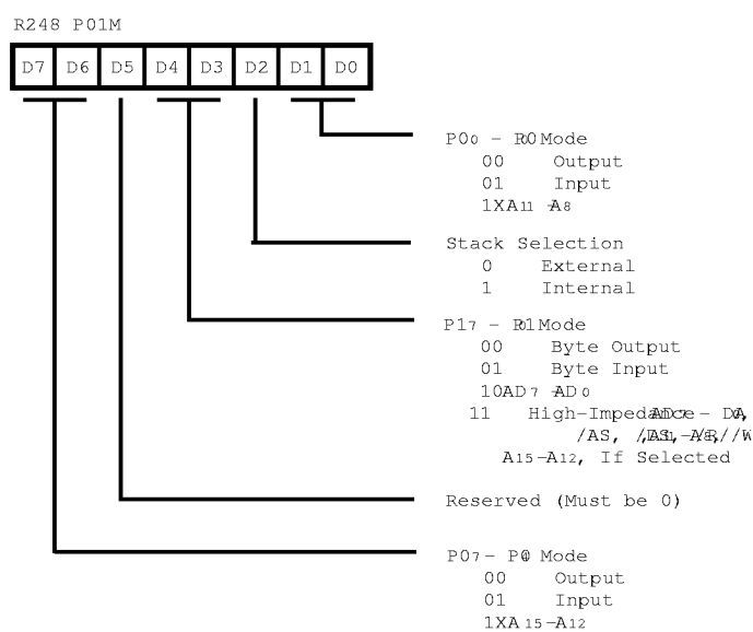
Figure 38. Port 0 and 1 Mode Register (F8 H : Write Only)
