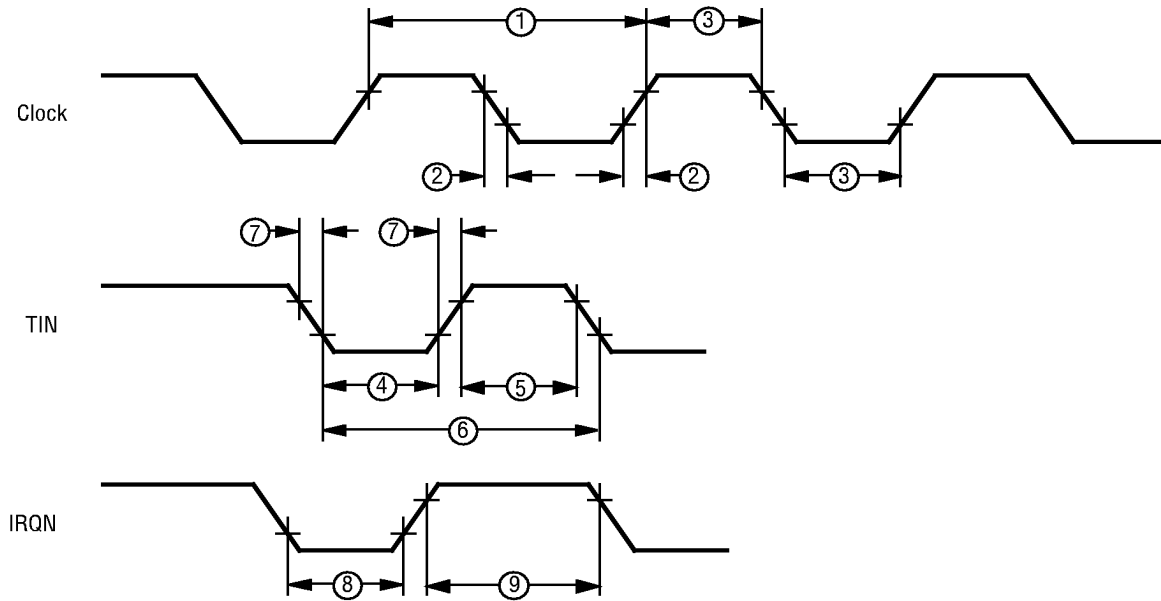
Figure 27. Additional Timing
