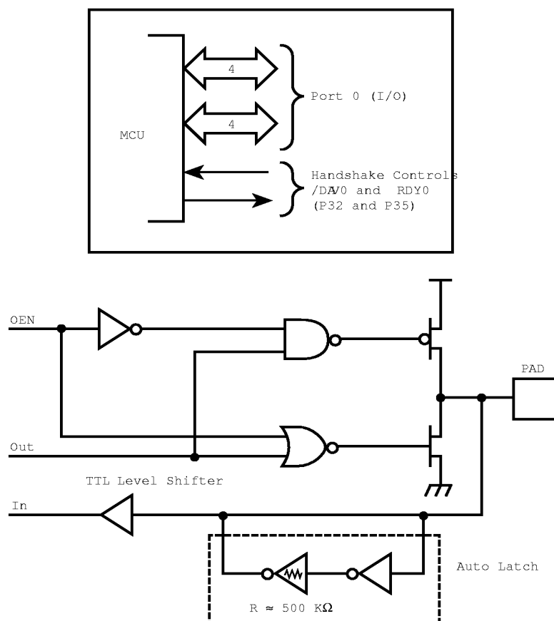
Figure 10. Port 0 Configuration
