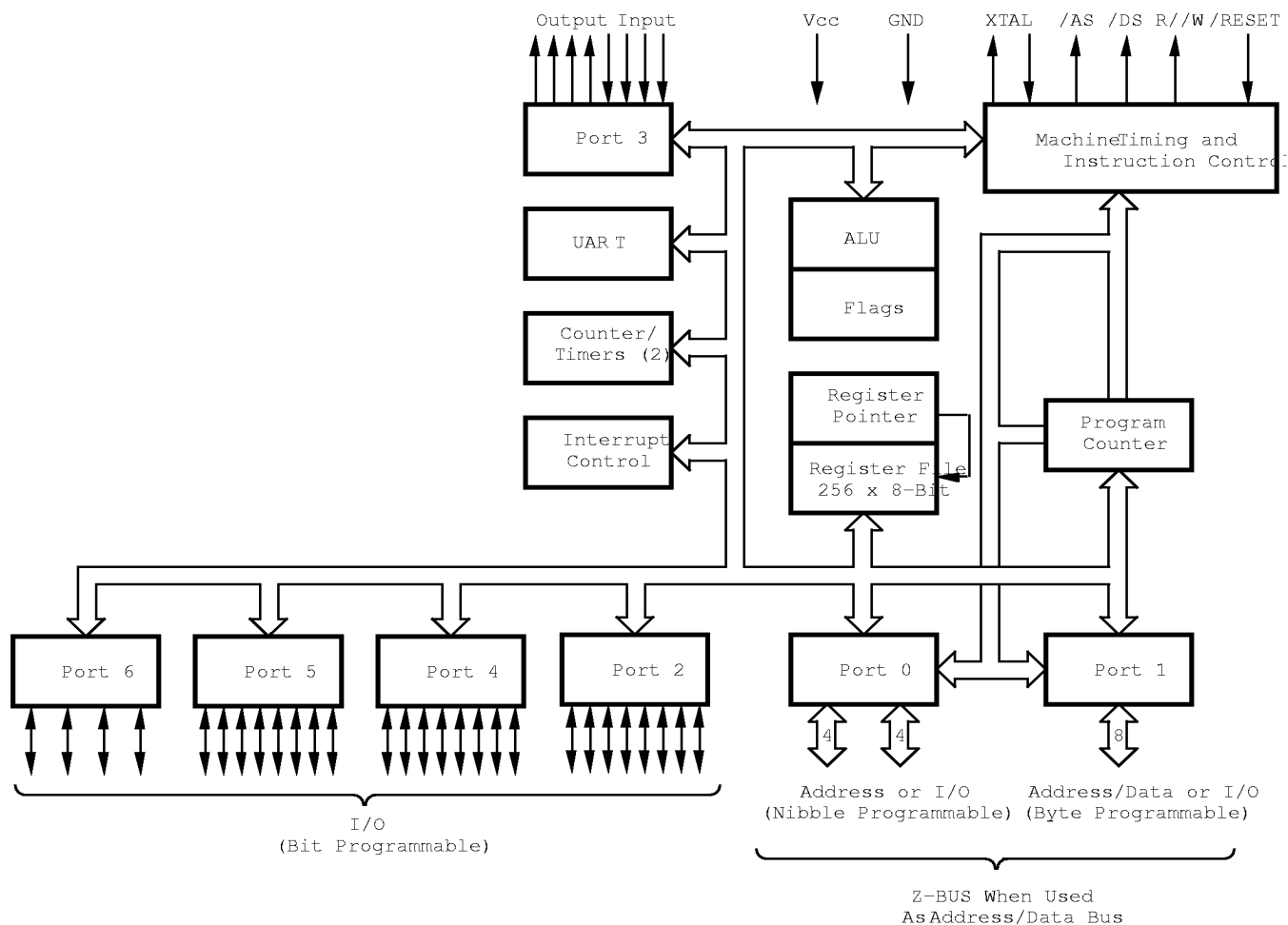
Figure 3. Z86C96 Functional Block Diagram
