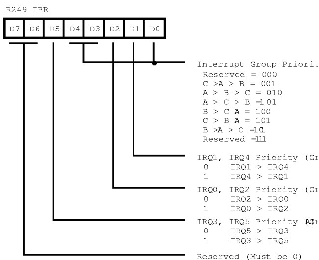
Figure 39. Interrupt Priority Register (F9 H : Write Only)
