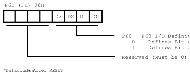
Figure 52. Port 6 Direction Register (F)08: (Write Only)
