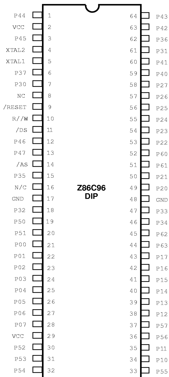
Figure 8. Z86C96 64-Pin DIP Pin Assignments
