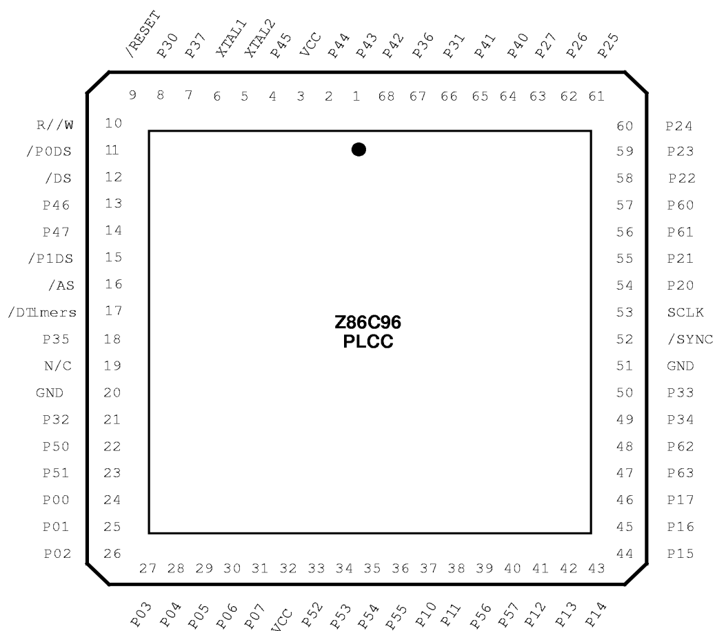
Figure 9. Z86C96 68-Pin PLCC Pin Assignments
