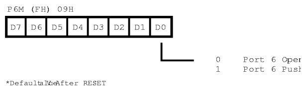
Figure 53. Port 6 Mode Register (F)09: (Write Only)
