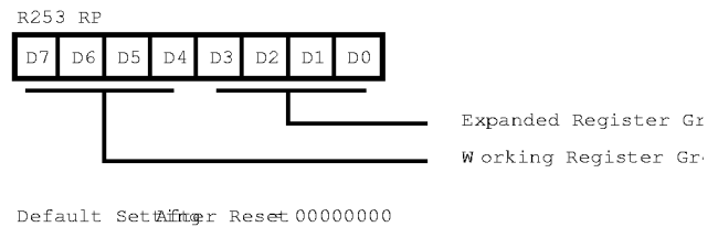
Figure 19. Register Pointer Register
