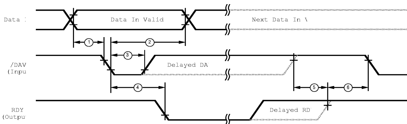
Figure 28. Input Handshake Timing
