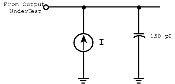
Figure 25. Test Load Diagram
