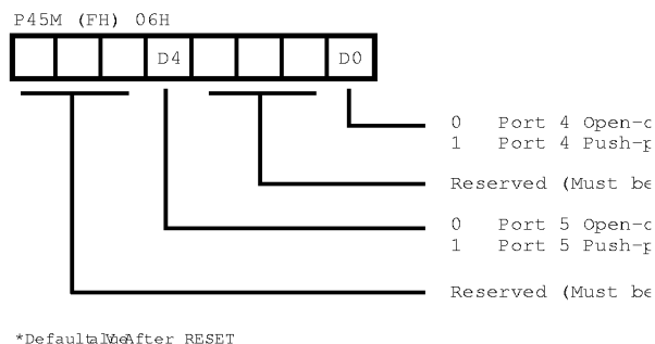
Figure 50. Port 4/5 Mode Register (F)06: (Write Only)
