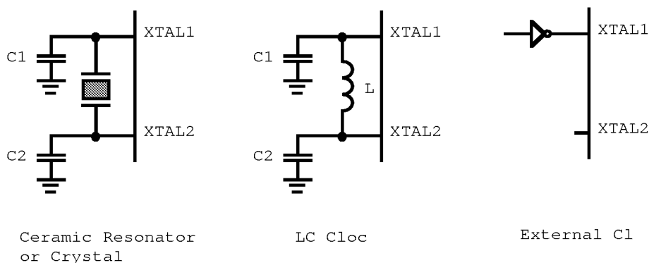
Figure 24. Oscillator Configuration
