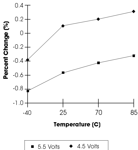
Chart 4: Oscillator Stability
