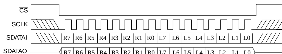
Figure 3-3 CS3310 Stereo Digital Volume Control
