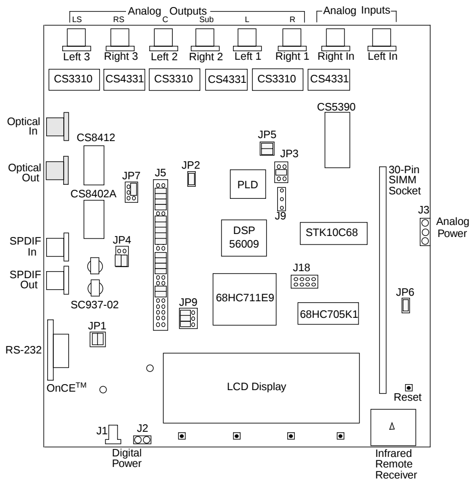
Figure A-3 DSP56009EVM Pass-through Setup
