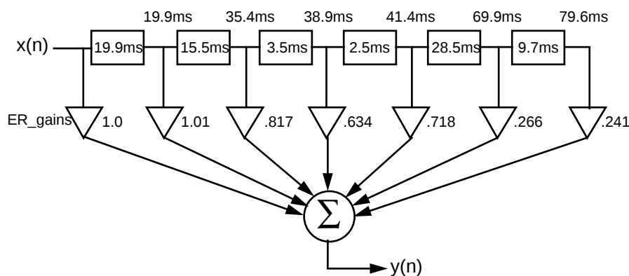
Figure B-2 Early Reflection FIR Block (one channel)
