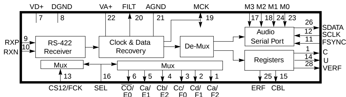
Figure 3-5 CS8412 Digital Audio Interface Receiver
