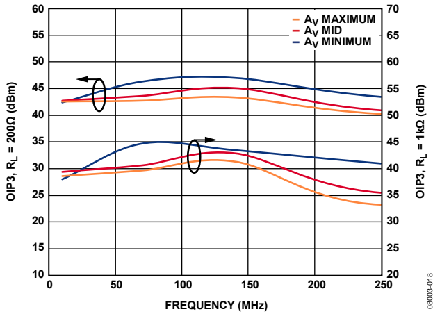
Figure 9. Output Third-Order Intercept at Three Gains, Output Level at 2 V p-p Composite, R_L = 200\ \Omega and 1\ k\Omega
