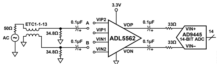
Figure 37. Wideband ADC Interfacing Example Featuring the AD9445
