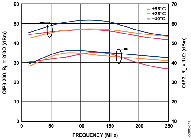
Figure 10. Output Third-Order Intercept vs. Frequency, Over Temperature, Output Level at 2 V p-p Composite, R_L = 200\ \Omega and 1\ k\Omega
