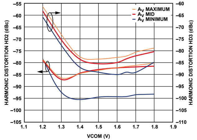
Figure 24. HD2/HD3 vs. VCOM
