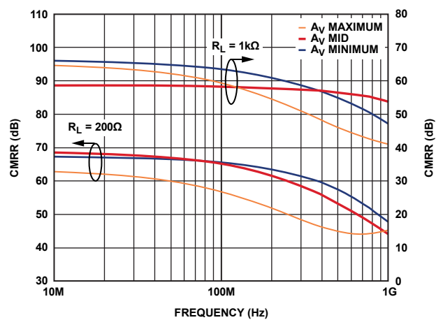
Figure 26. Common-Mode Rejection Ratio vs. Frequency
