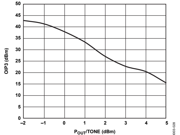
Figure 13. Output Third-Order Intercept vs. Power, Frequency 140 MHz, A_v = 15.5\ dB
