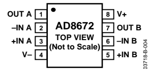
Figure 4. 8-Lead MSOP (RM Suffix)
