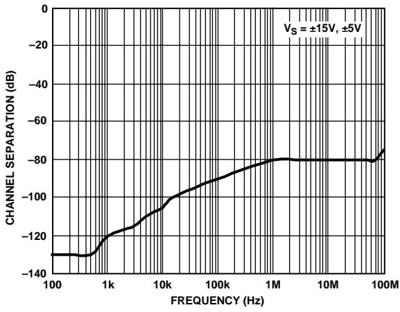
Figure 31. Channel Separation
