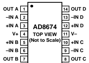
Figure 5. 14-Lead SOIC (R Suffix)
