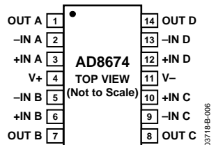
Figure 6. 14-Lead TSSOP (RU Suffix)
