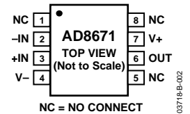
Figure 2. 8-Lead MSOP (RM Suffix)
