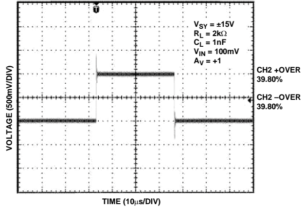
Figure 36. Capacitive Load Drive
