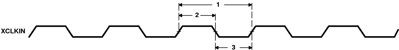
Figure 9. XCLKIN Timings
