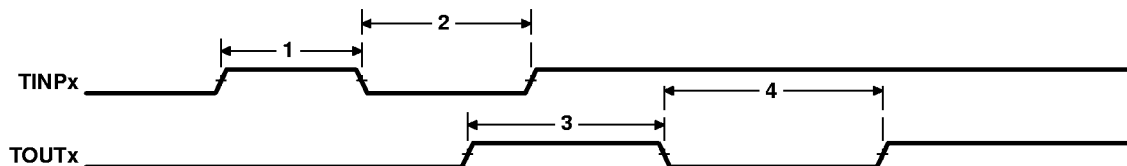
Figure 50. Timer Timing
