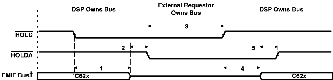
Figure 24. HOLD/HOLDA Timing
