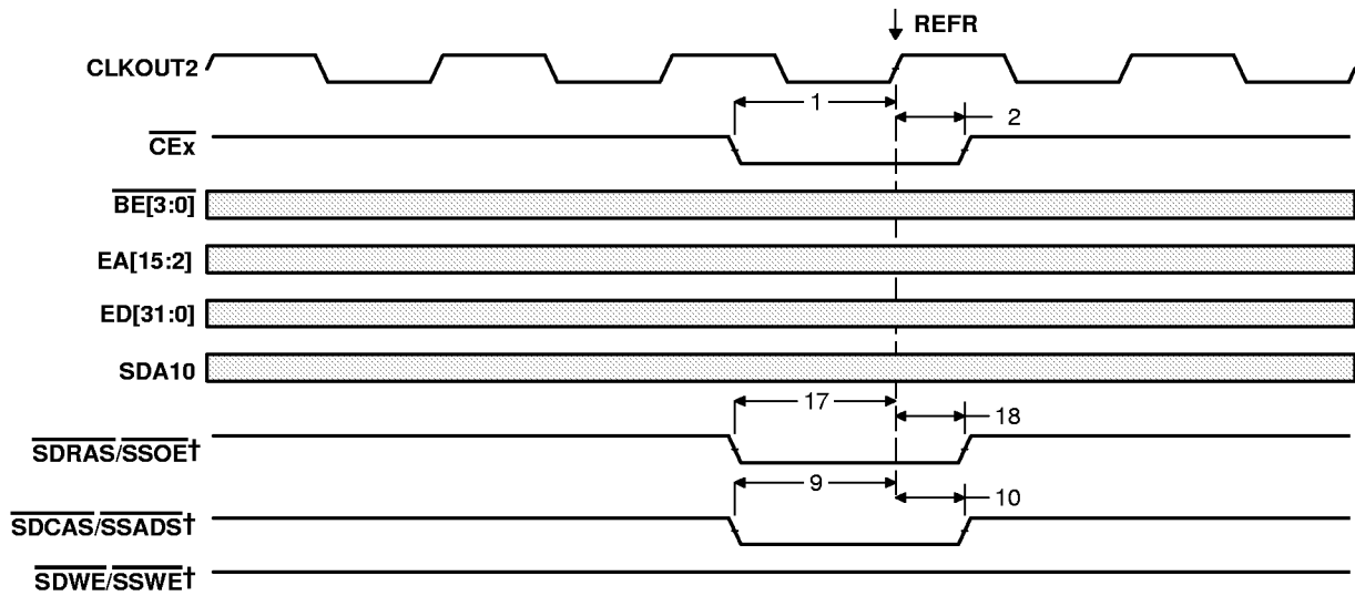
Figure 22. SDRAM REFR Command
