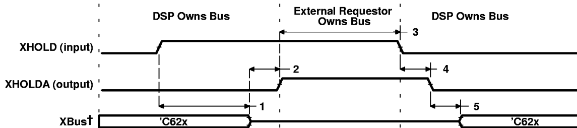
Figure 41. Expansion Bus Arbitration—Internal Arbiter Enabled
