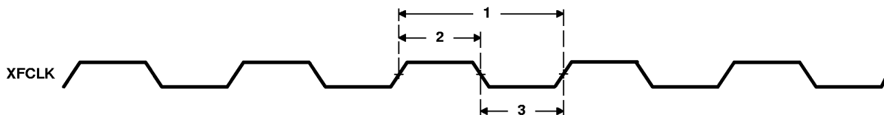
Figure 11. XFCLK Timings
