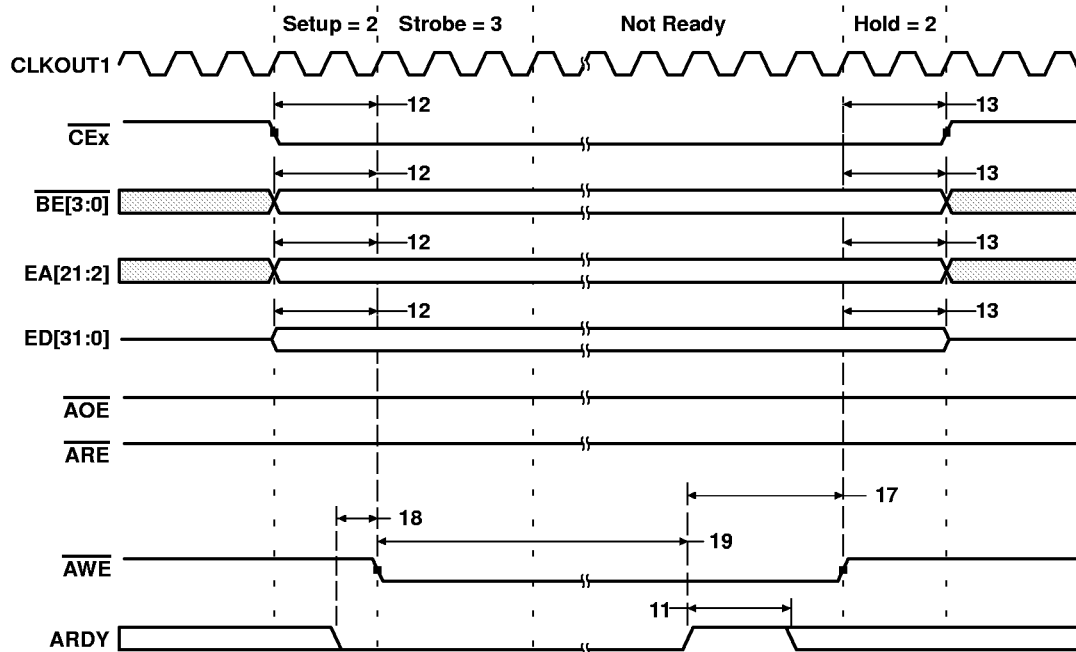
Figure 15. Asynchronous Memory Write Timing (ARDY Used)
