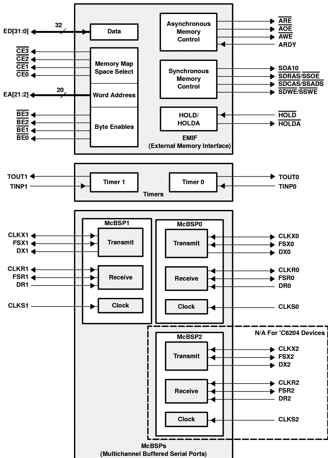
Figure 3. Peripheral Signals
