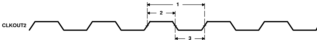
Figure 10. CLKOUT2 Timings
