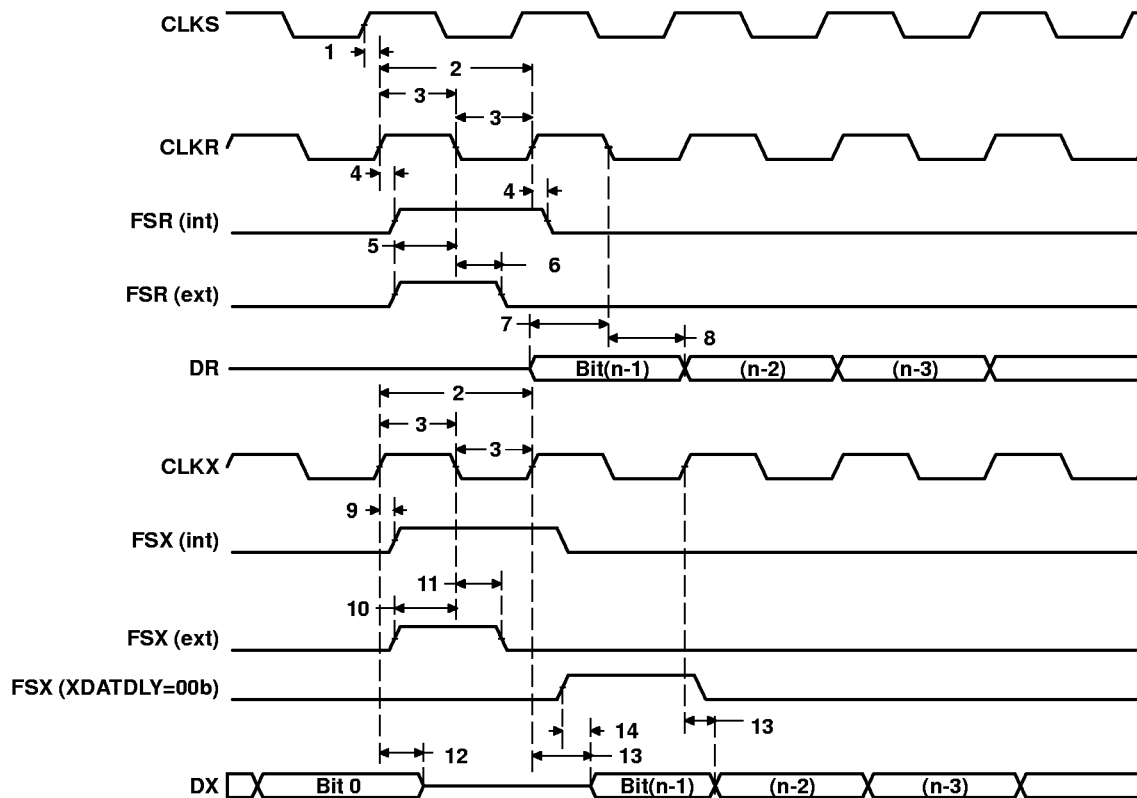
Figure 43. McBSP Timings
