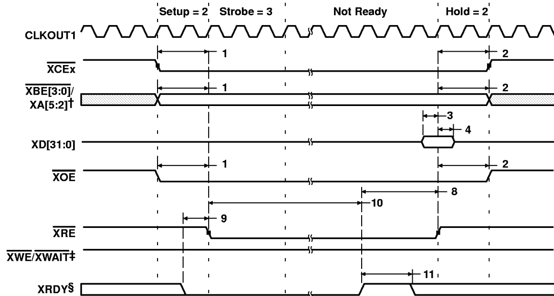
Figure 30. Expansion Bus Asynchronous Peripheral Read Timing (XRDY Not Used)
