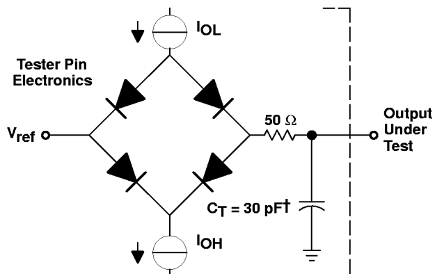
Figure 6. Test Load Circuit
