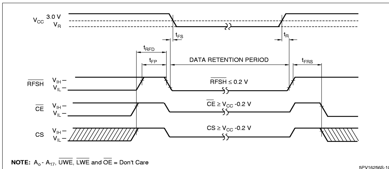
Figure 11. Data Retention Mode
