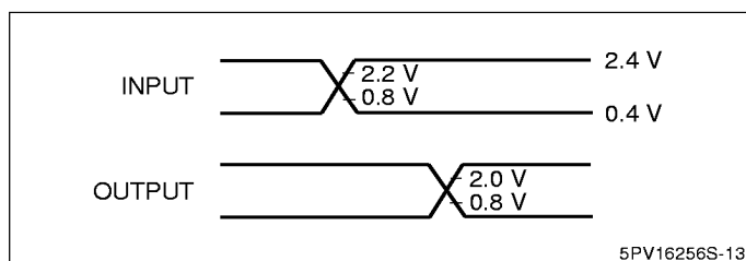
Figure 3. AC Characteristics
