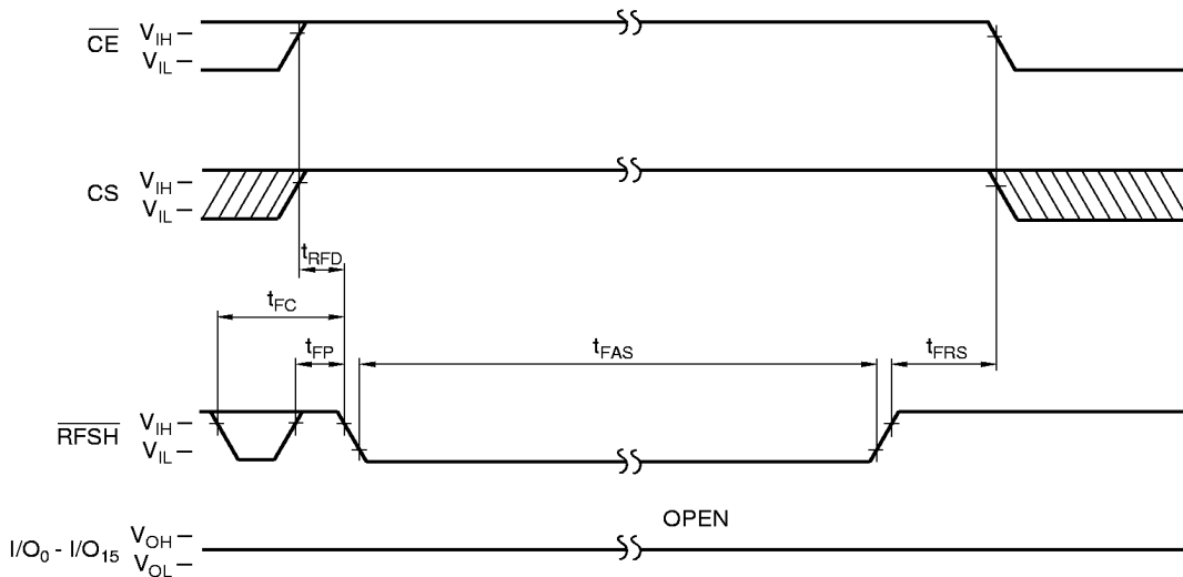
Figure 10. Self Refresh Cycle
