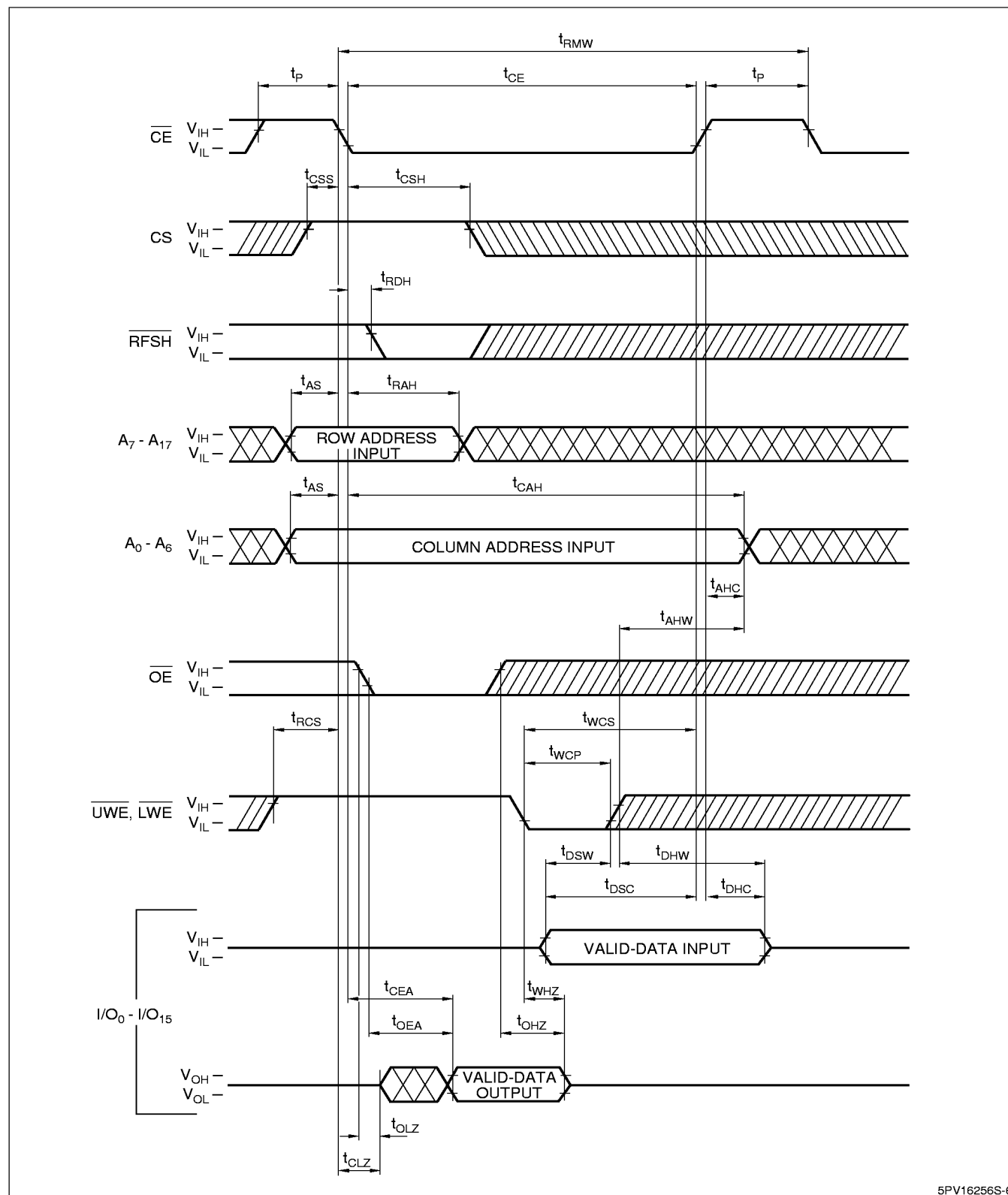
Figure 7. Read-Modify-Write Cycle
