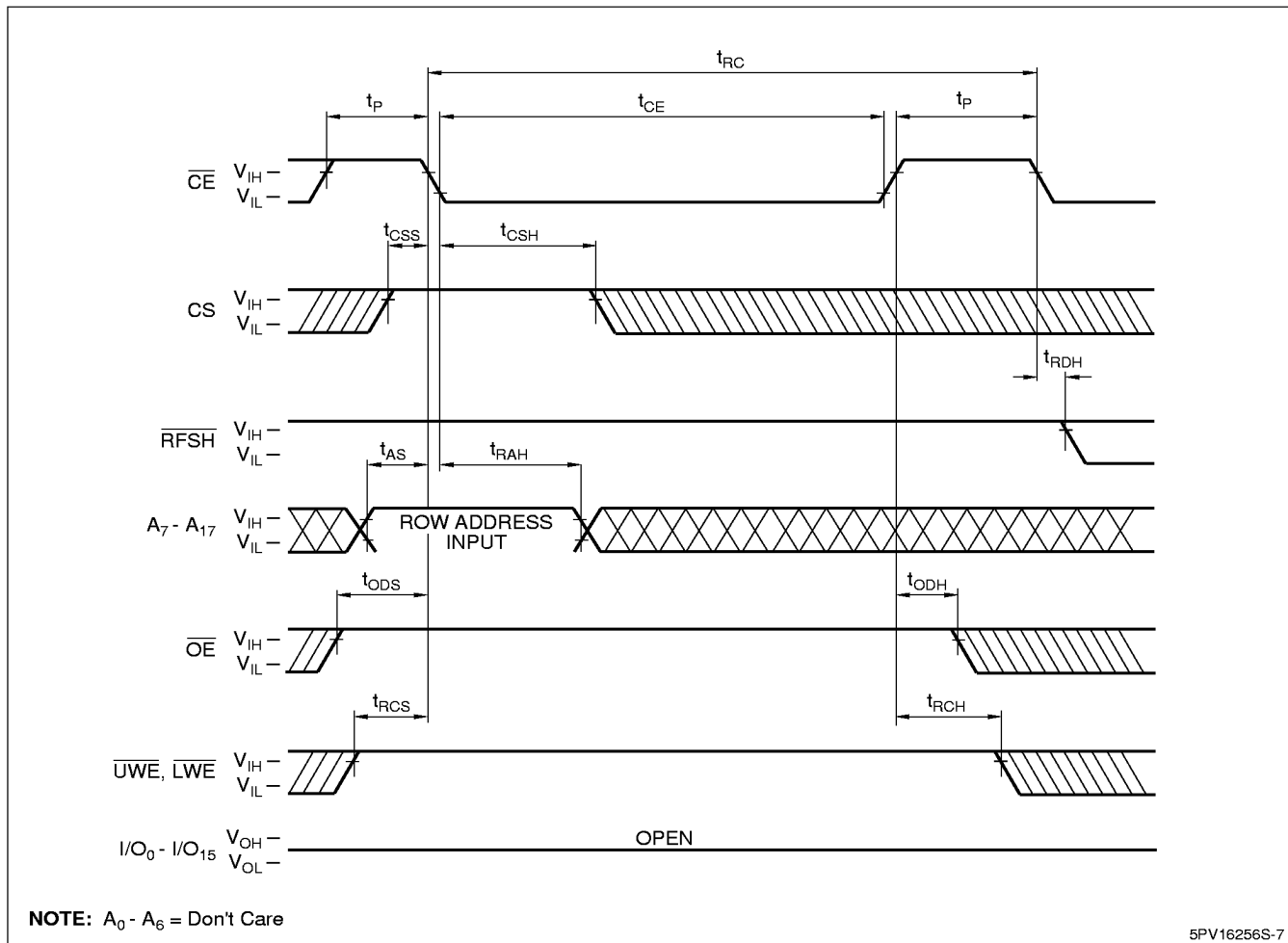
Figure 8. Address Refresh Cycle
