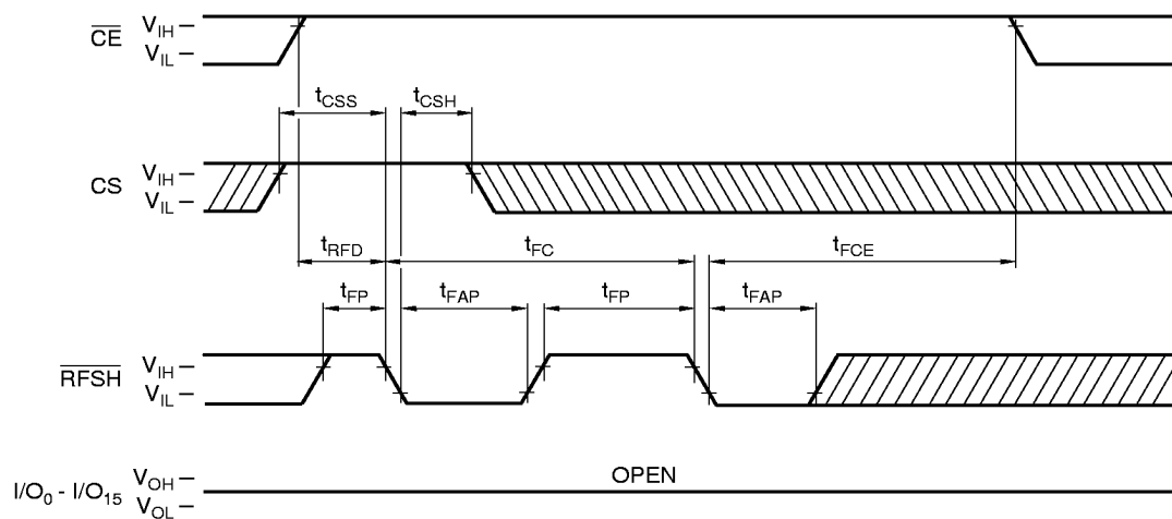
Figure 9. Auto Refresh Cycle
