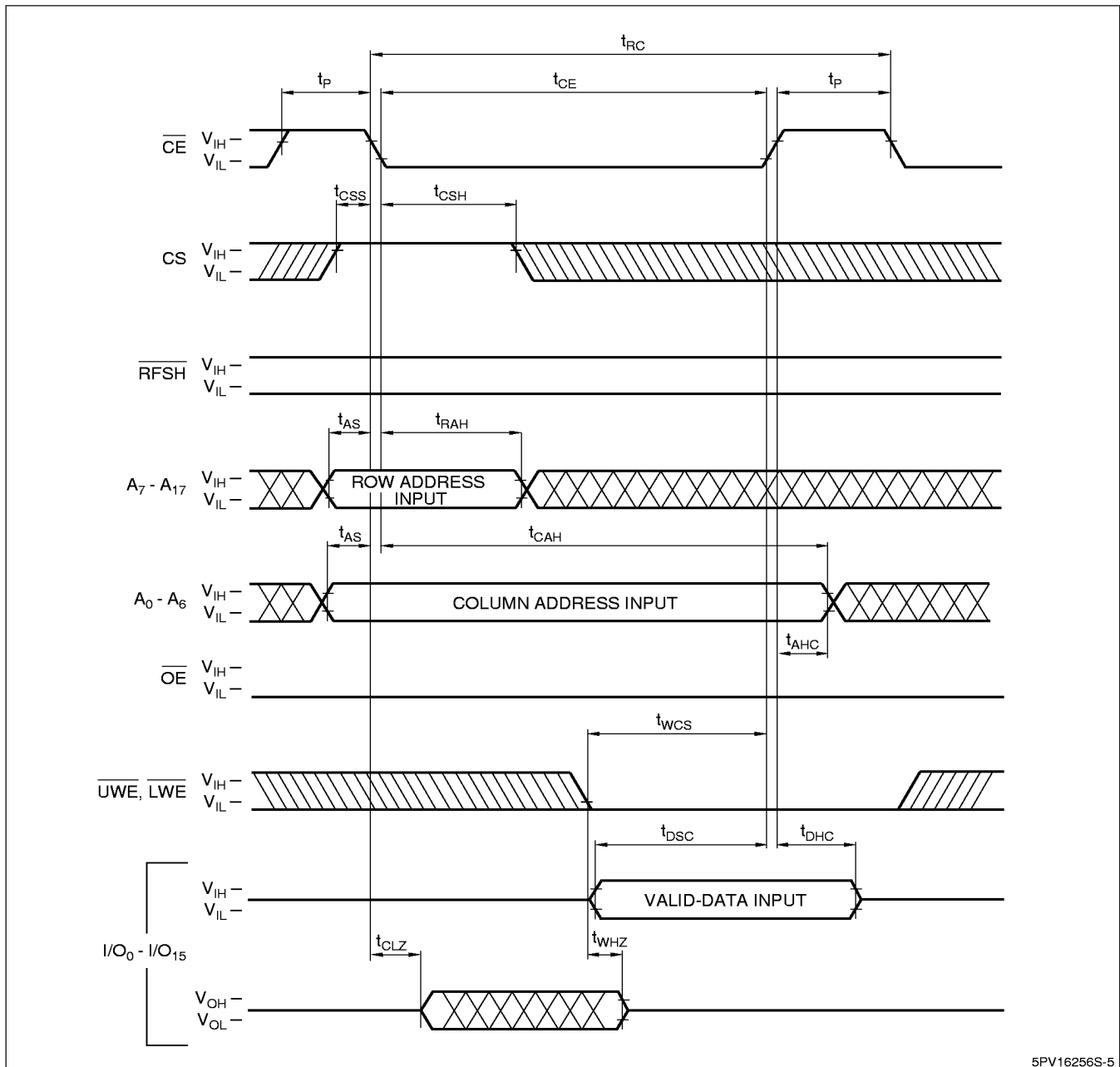
Figure 6. Write Cycle (2) (OE = Low , CE Control)
