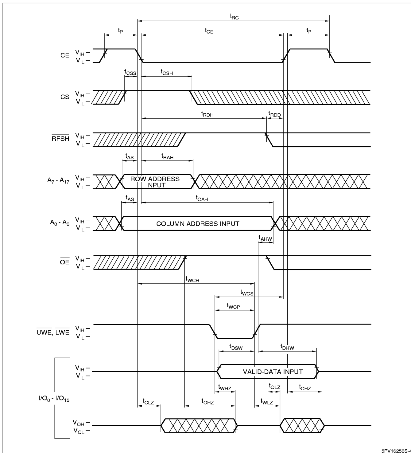
Figure 5. Write Cycle (1) (OE Clock)
