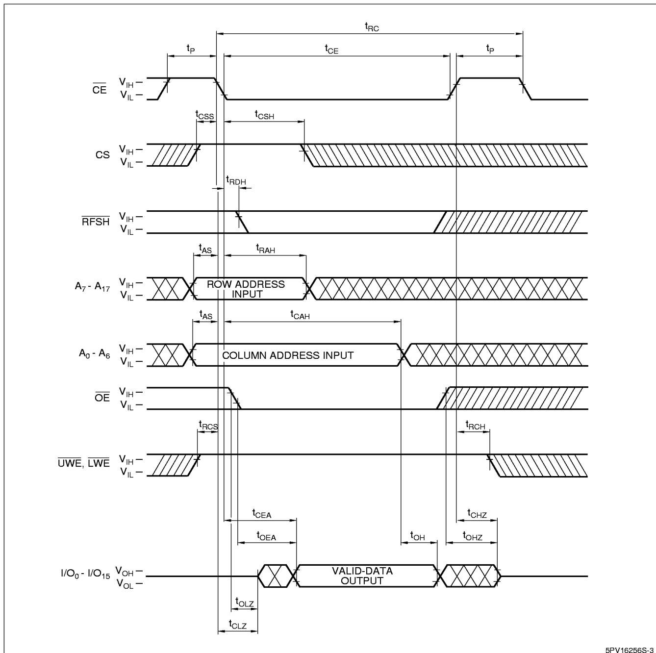
Figure 4. Read Cycle
