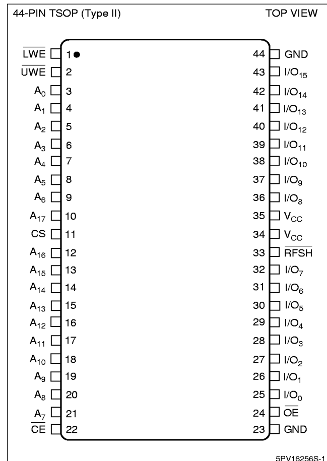
Figure 1. Pin Connections
