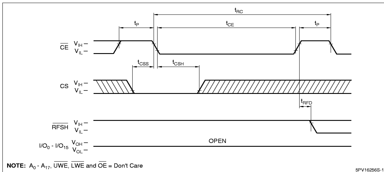
Figure 12. CS Standby Mode
