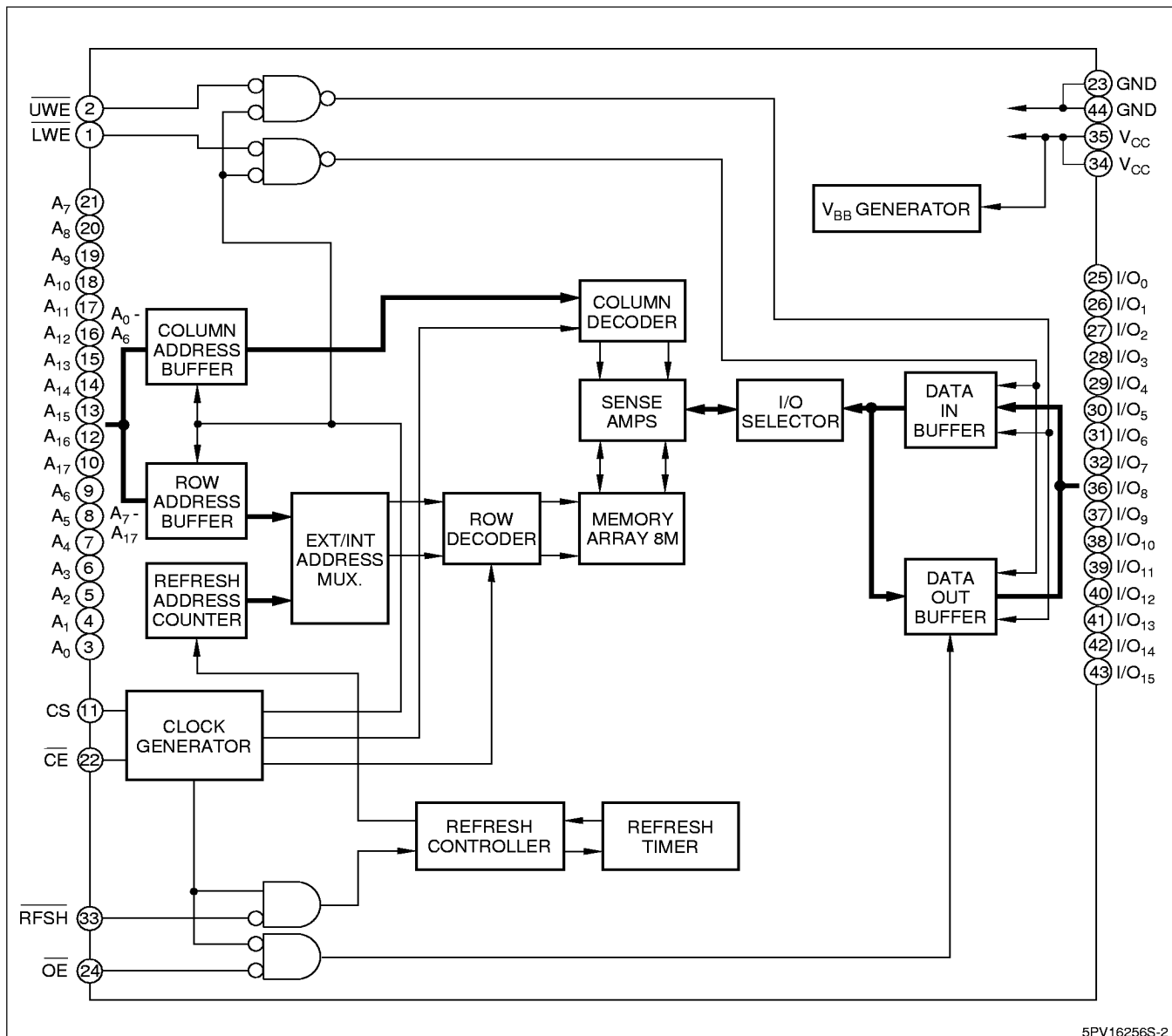
Figure 2. LH5PV16256 Block Diagram
