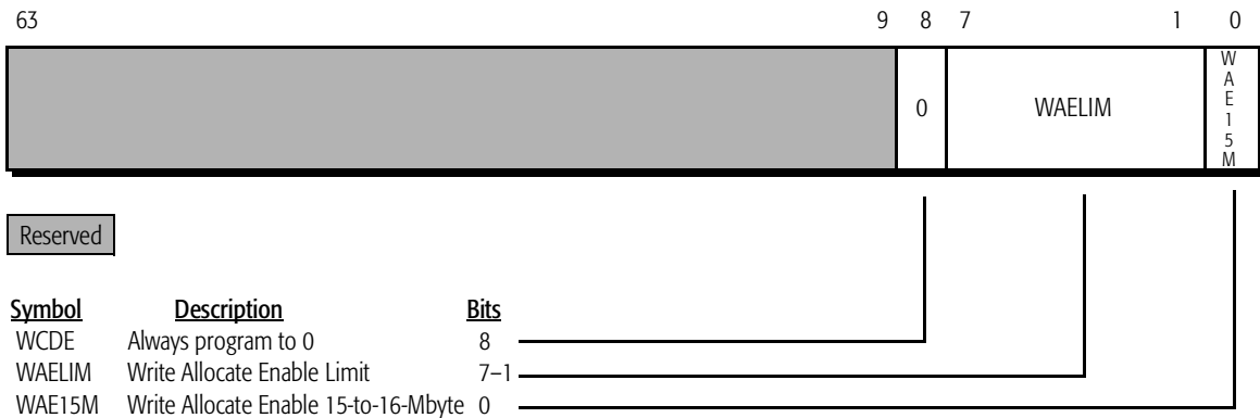
Figure 36. Write Handling Control Register (WHCR)—Model 8/[7:0]
