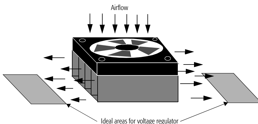
Figure 109. Airflow for a Heatsink with Fan
