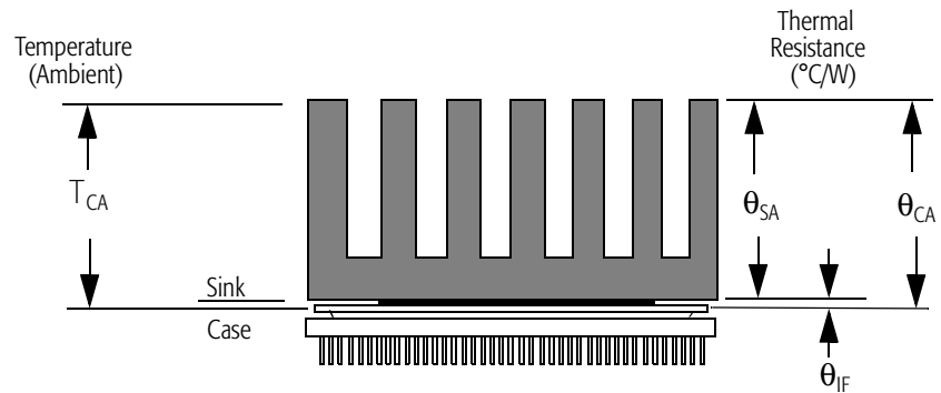
Figure 104. Thermal Model
