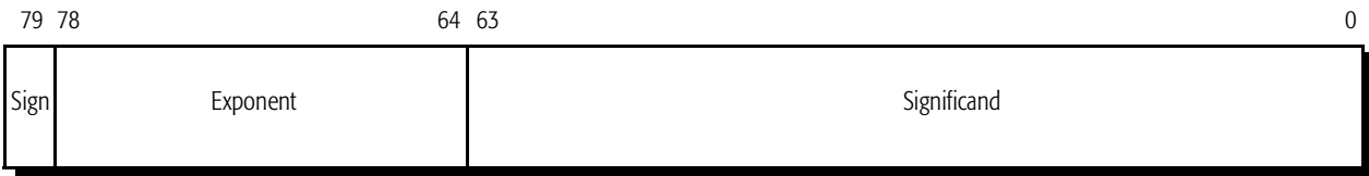
Figure 11. Floating-Point Register
