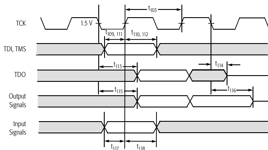
Figure 103. Test Signal Timing Diagram
