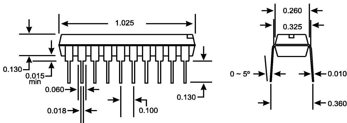
20 PIN DIP Package
