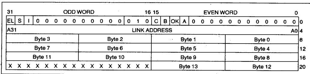
Figure 25. CONFIGURE—Linear Mode
