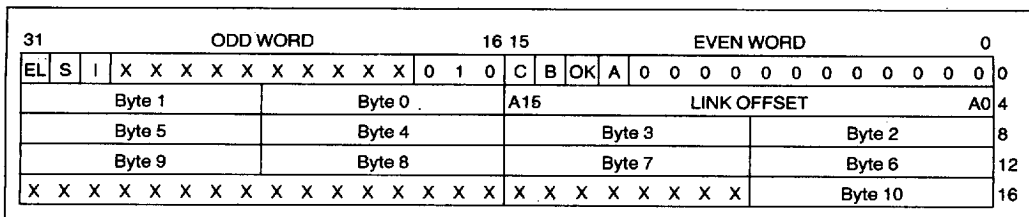
Figure 23. CONFIGURE—82586 Mode
