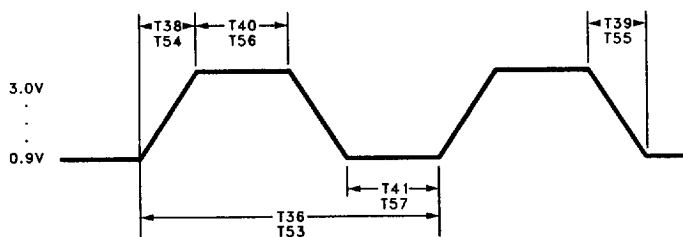
Figure 56. Serial Input Clock Timing
