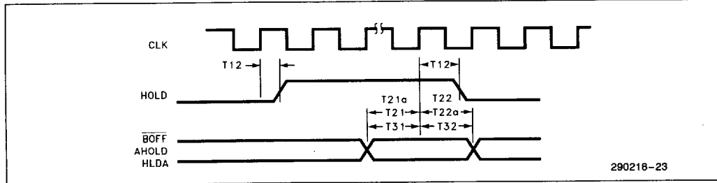
Figure 50. HOLD/HLDA Timings
