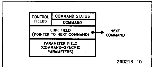
Figure 10. Action Command Format
