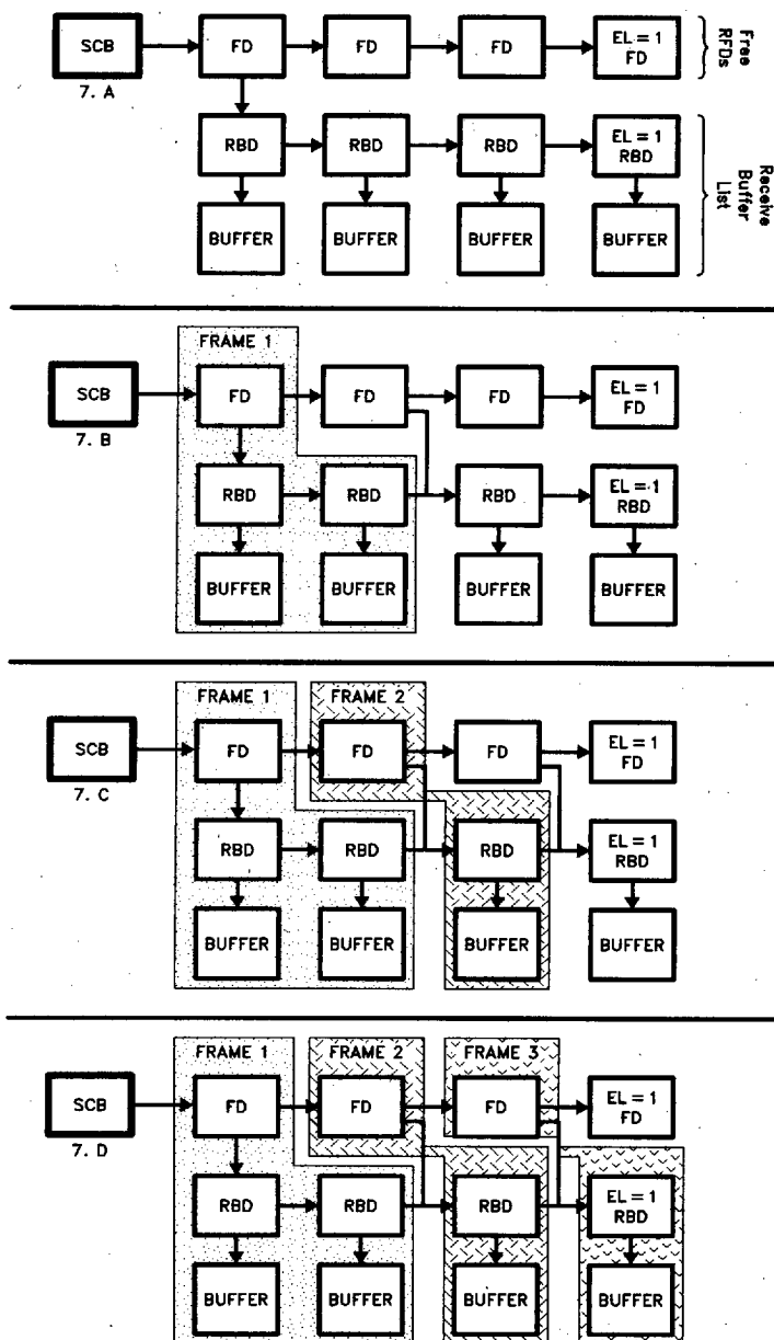
Figure 7. Frame Reception in the RFA
