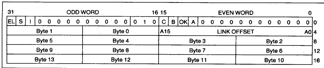
Figure 24. CONFIGURE—32-Bit Segmented Mode
