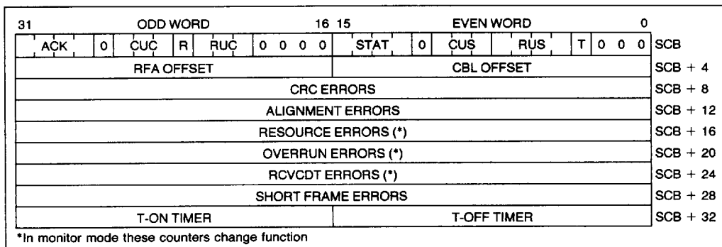
Figure 19. SCB—32-Bit Segmented Mode
