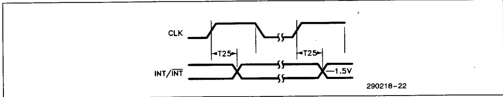
Figure 49. INT/INT Output Timing
