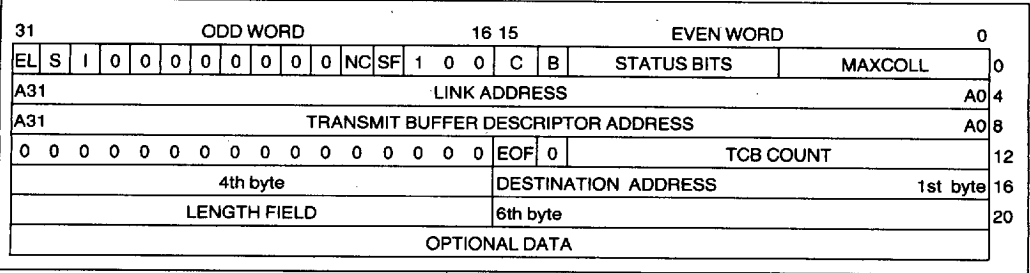
Figure 30. TRANSMIT—Linear Mode
