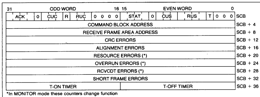
Figure 20. SCB—Linear Mode
