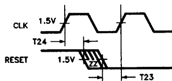
Figure 55. RESET Input Timing
