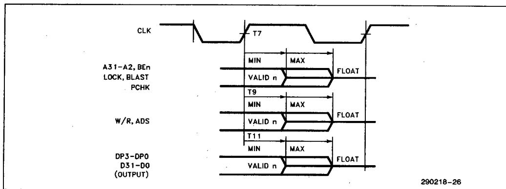
Figure 53. Output Float Delay Timing
