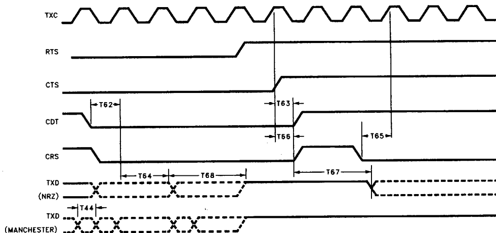
Figure 57. Transmit Data Waveforms
