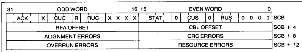
Figure 18. SCB—82586 Mode
