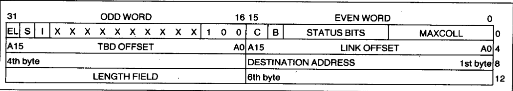
Figure 28. TRANSMIT—82586 Mode
