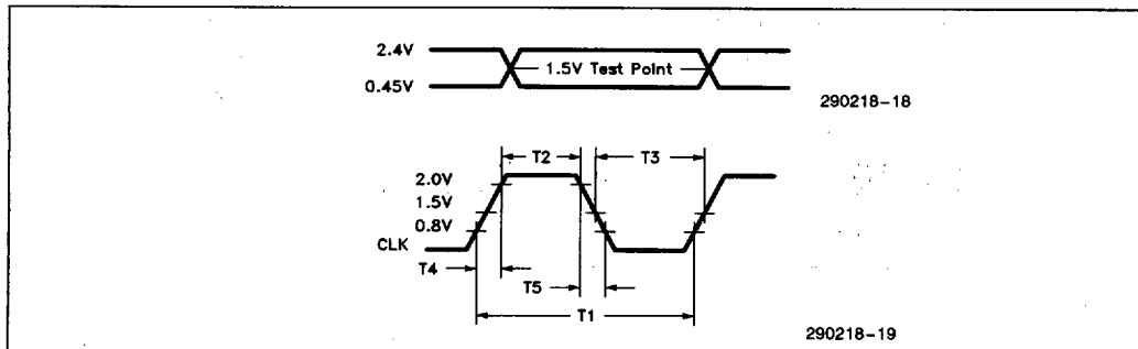
Figure 46. CLK Timings
