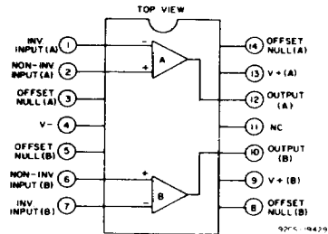
1f. —CA747CE and CA747E with internal phase compensation.
