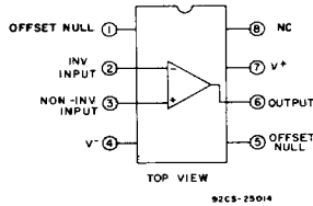
1e. —CA741C and CA741E with internal phase compensation.
