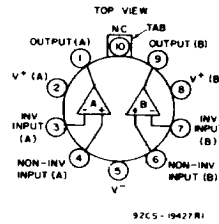
1b. —CA747CT and CA747T with internal phase compensation.
