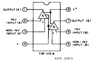
1h. —CA1458E and CA1558E with internal phase compensation.
