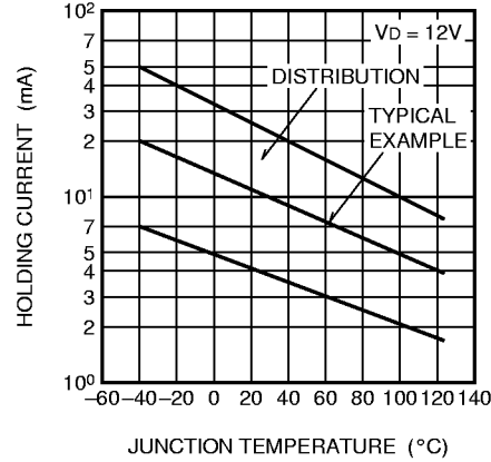
HOLDING CURRENT VS. JUNCTION TEMPERATURE
