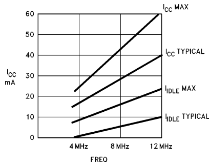
Figure 4. I_{CC} and I_{IDLE} vs Frequency
