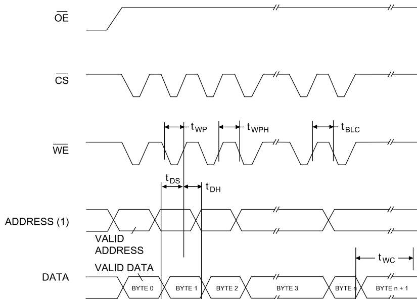
FIG. 9 PAGE WRITE WAVEFORMS
