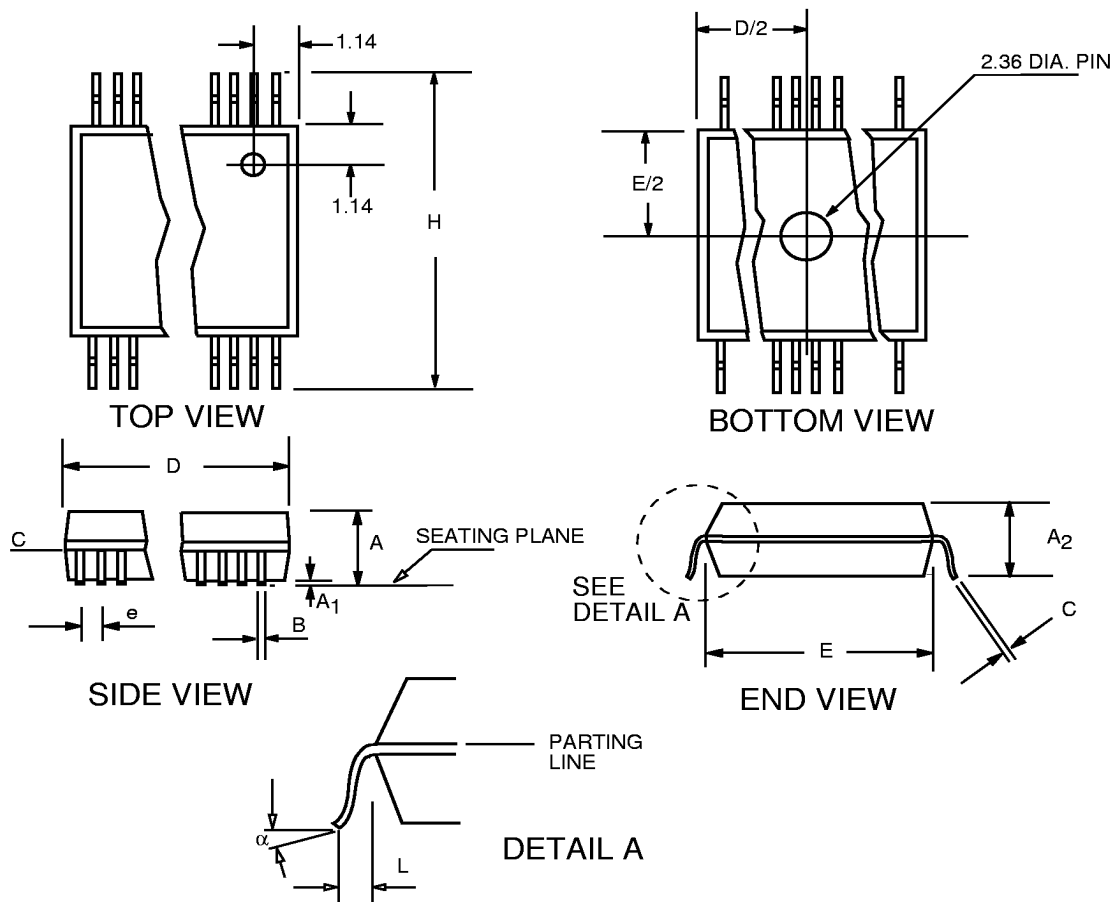
SSOP Package
