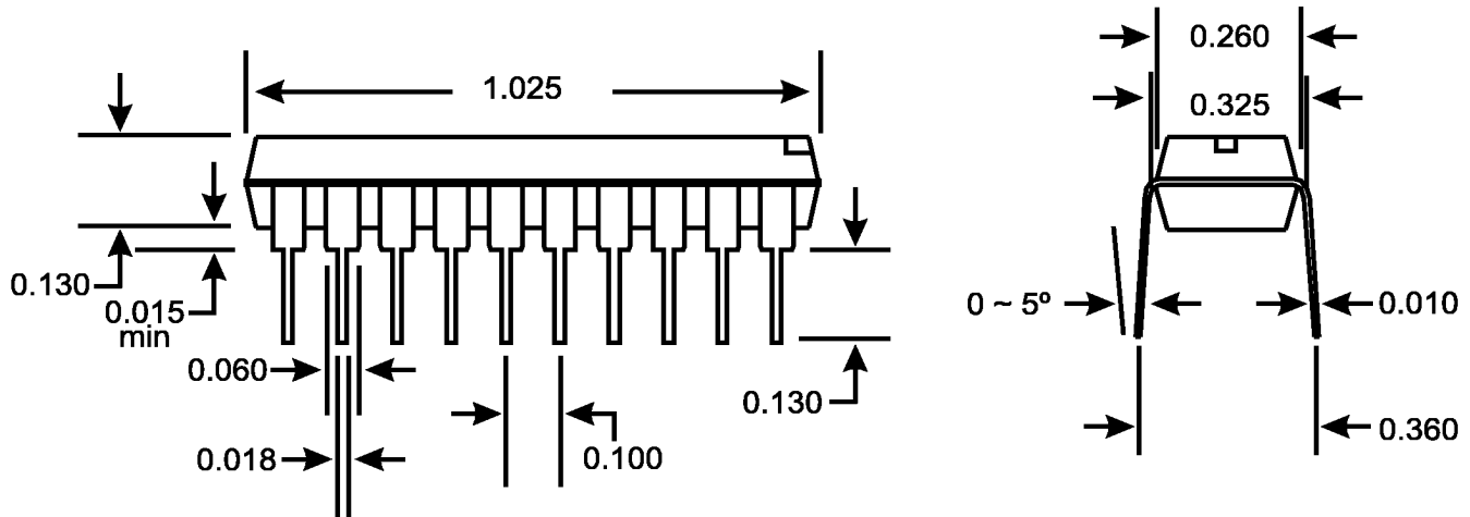
20-Pin DIP Package
