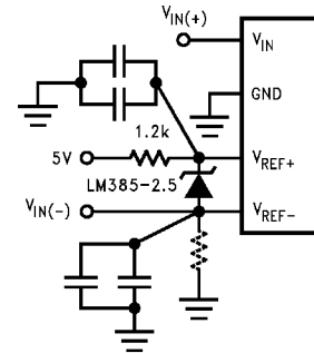
Input Not Referred to GND
