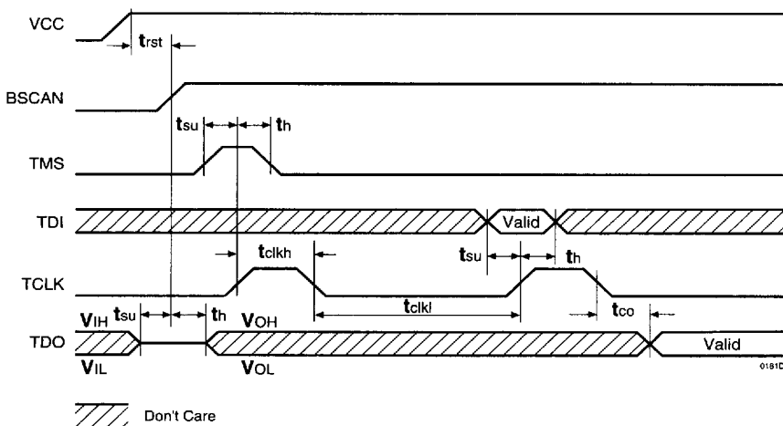
Figure 10. Boundary Scan Waveforms
