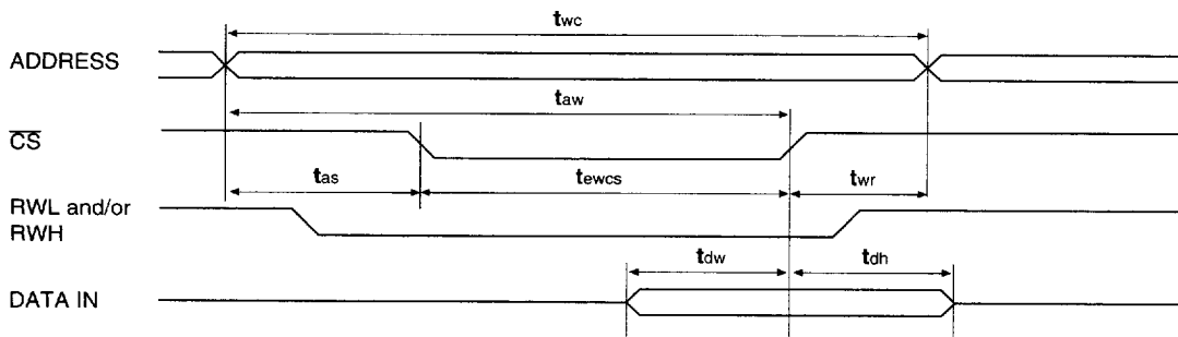
Figure 25. Dual Port RAM Write Cycle ( \overline{CS} Controlled) Timing Diagram
