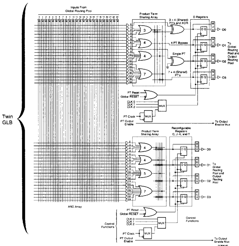
Figure 2. ispLSI and pLSI 6192 Twin GLB
