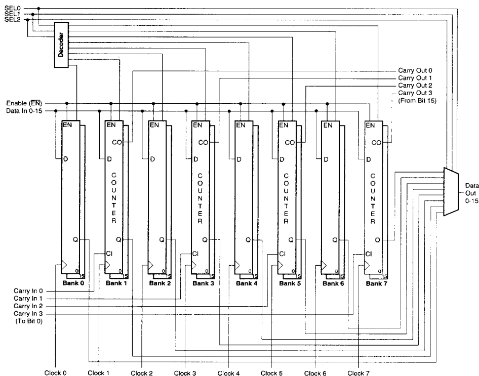
Figure 41. Register/Counter Option #5: 4 Bank Parallel Load Up/Down Counter with 4 Bank Register File
