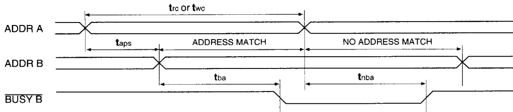
Figure 23. Dual Port RAM Contention Cycle (Address Valid Arbitration) Timing Diagram
