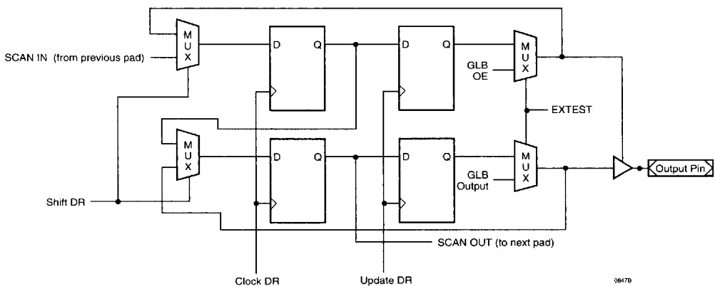
Figure 9. Boundary Scan Registers for Output-Only Cell
