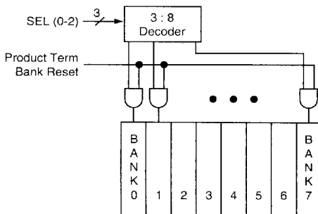
Figure 33. Product Term Bank Reset
