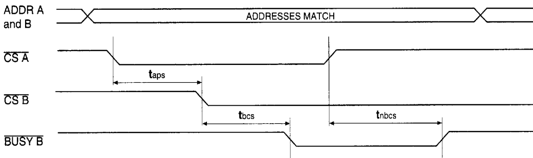
Figure 22. Dual Port RAM Contention Cycle ( \overline{CS} Arbitration) Timing Diagram
