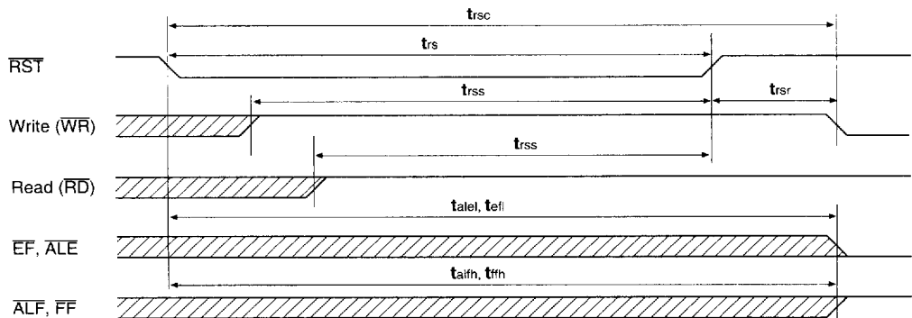
Figure 16. FIFO Reset Timing Waveform
