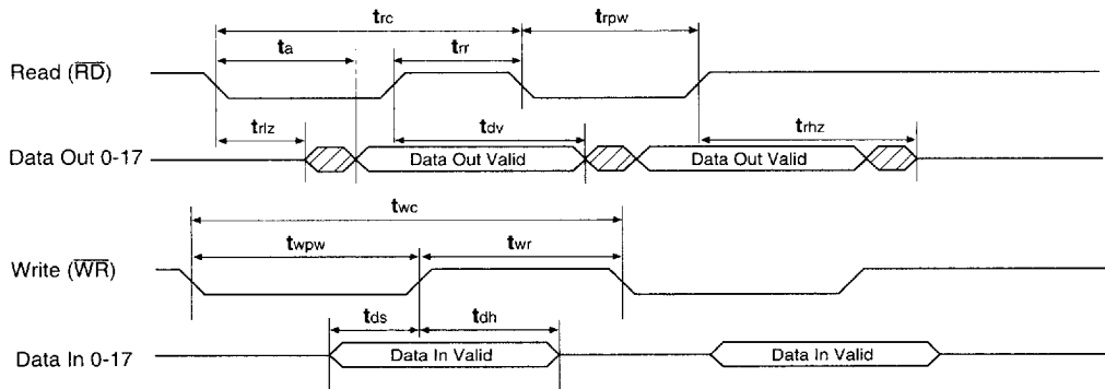
Figure 15. Asynchronous Write and Read Operation Timing Waveform
