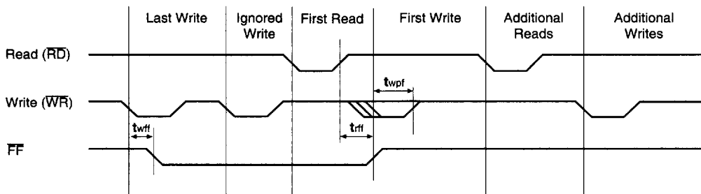
Figure 12. Full Flag from Last Write Timing Waveform
