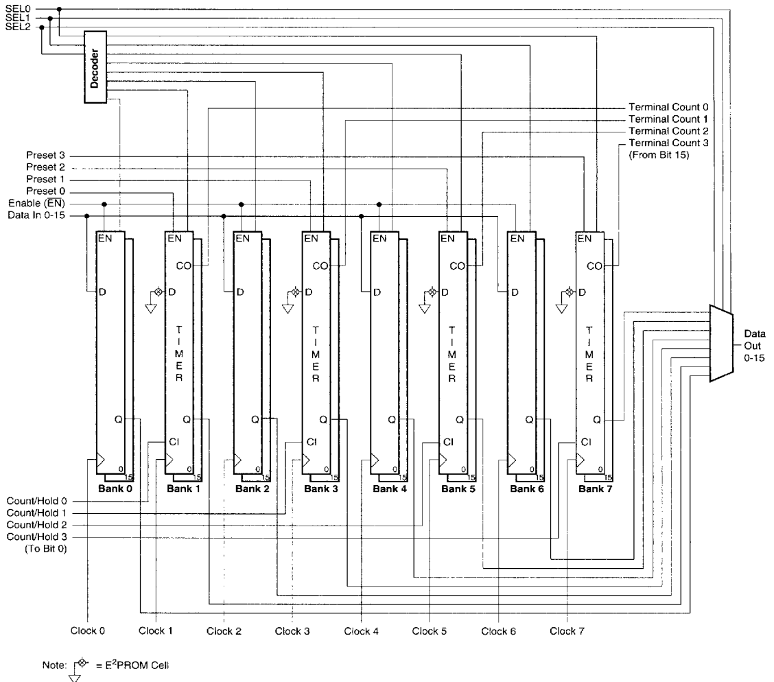
Figure 46. Register/Counter Option #9: 4 Bank Custom Preset Load Up/Down Timer with 4 Bank Register File
