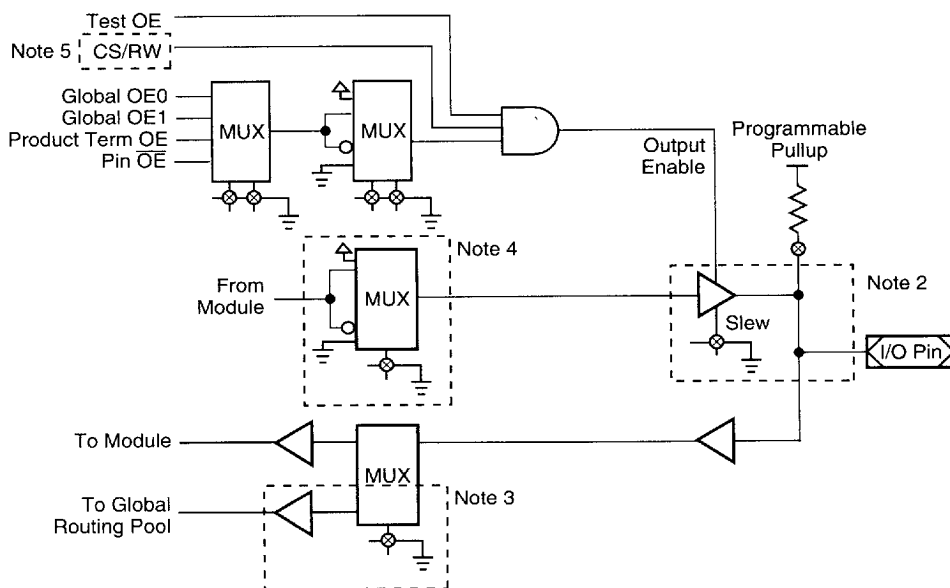
Figure 48. Module Bidirectional I/O cell
