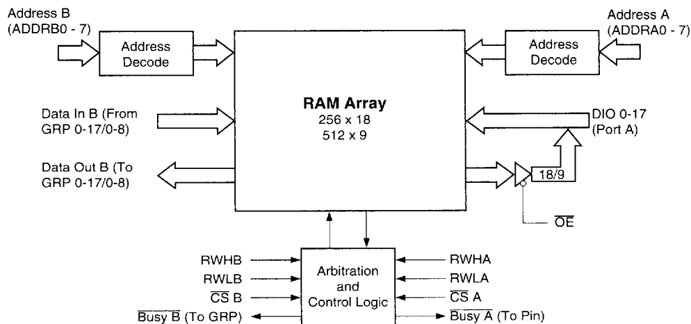
Figure 19. Dual Port RAM Functional Block Diagram
