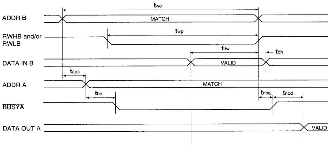
Figure 21. Dual Port RAM with Busy Timing Diagram
