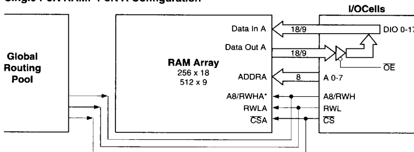
Figure 28. Single Port RAM: Port A Configuration
