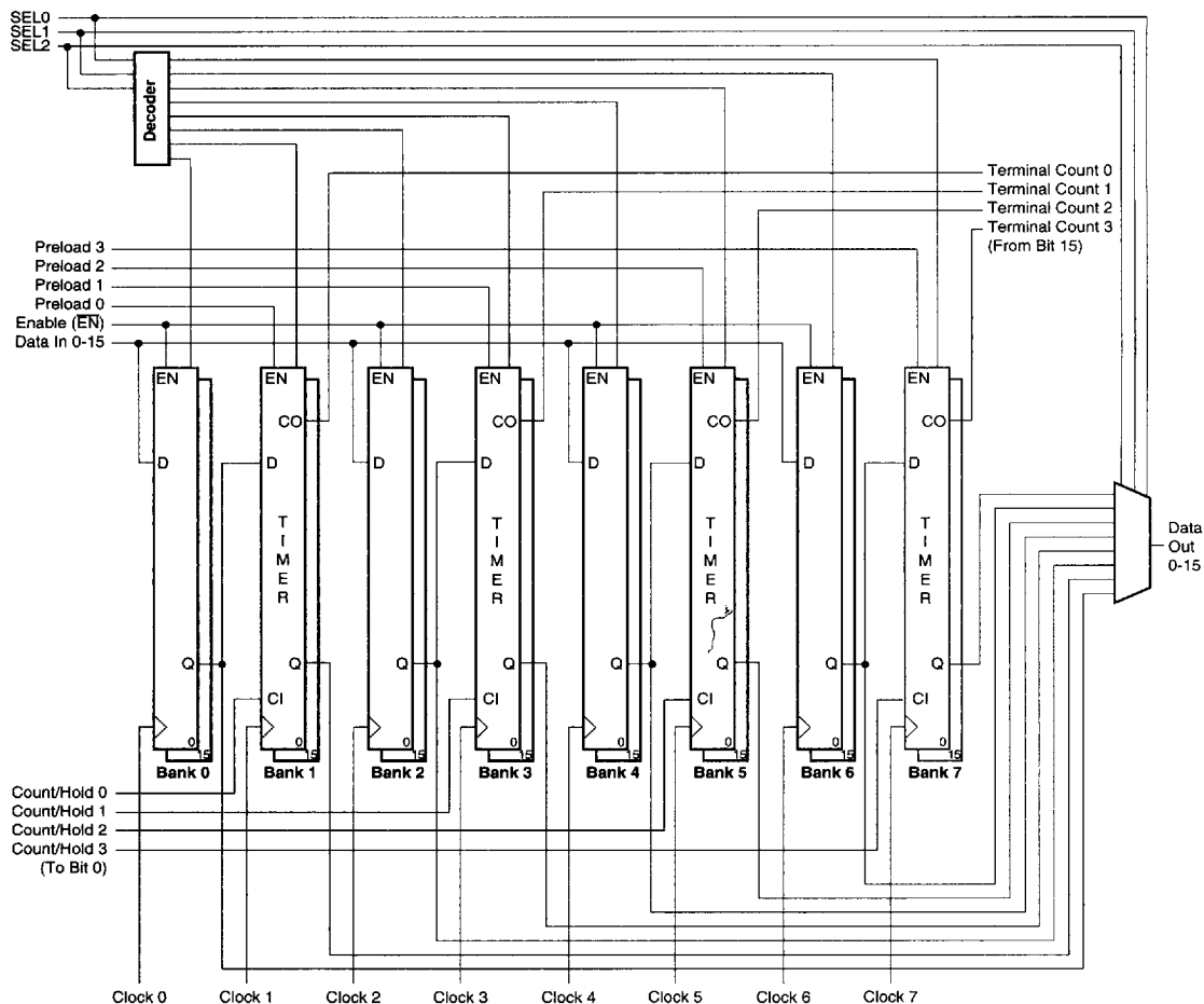
Figure 45. Register/Counter Option #8: 4 Bank Adjacent Load Up/Down Timer with 4 Bank Adjacent Register File
