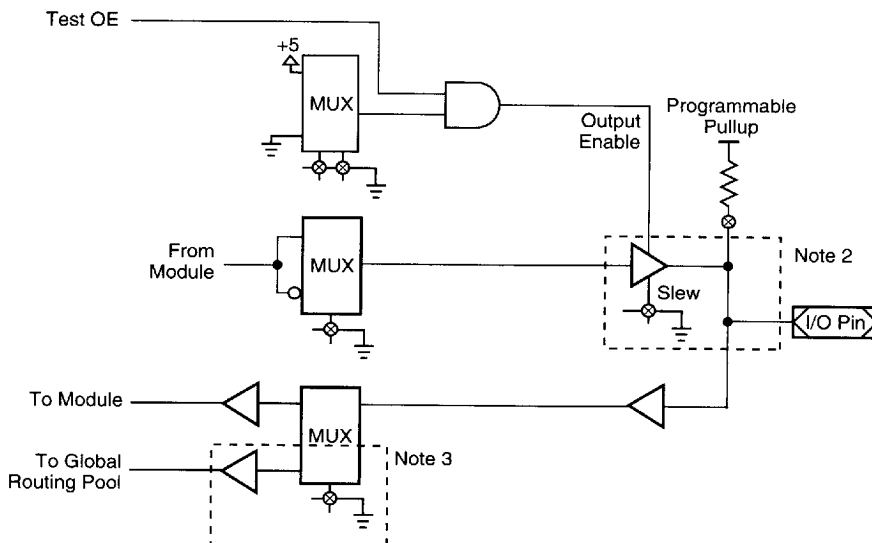
Figure 49. Module I/O Cell
