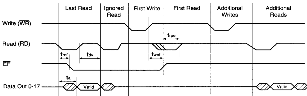
Figure 13. Empty Flag from Last Read Timing Waveform
