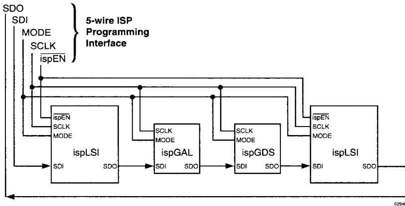
Figure 52. ISP™ Programming Interface
