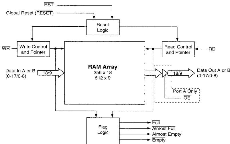
Figure 11. FIFO Module Functional Block Diagram
