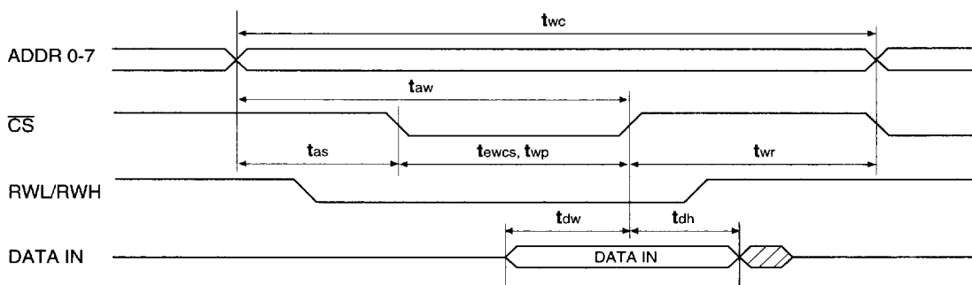
Figure 31. Single Port RAM Write Cycle (CS Controlled) Timing Diagram
