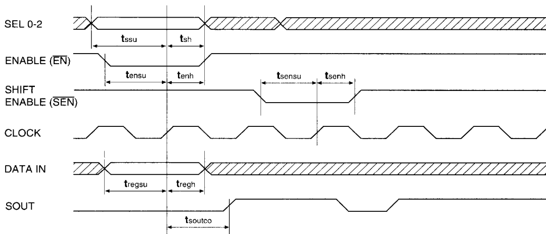
Figure 37. Shift Register Parallel Load/Shift Timing Diagram
