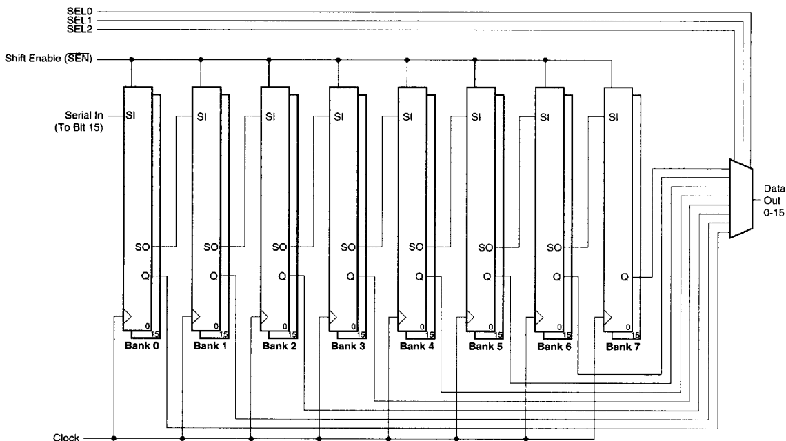
Figure 39. Register/Counter Option #3: 8-Bank Serial to Parallel Shift Register
