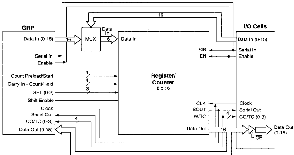
Figure 32. Register/Counter Module Connectivity
