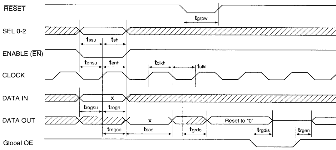
Figure 35. Register Parallel Read/Write Timing Diagram
