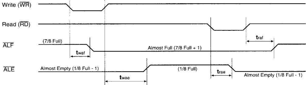
Figure 14. Almost-Empty/Almost-Full Flag Timing Waveform
