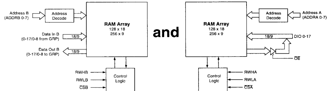
Figure 27. Single Port RAM Functional Block Diagram (Dual RAM Blocks)
