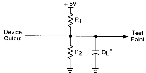
Figure 50. Test Load
