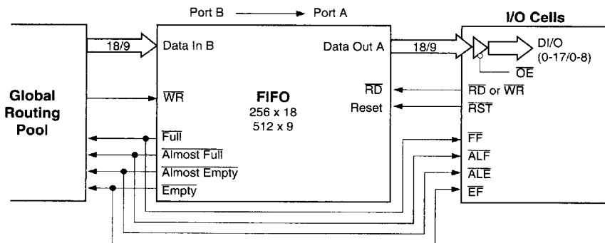
Figure 18. Port B to A Configuration
