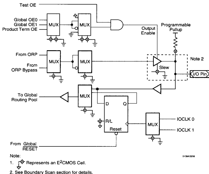
Figure 47. General-Purpose Bidirectional I/O Cell
