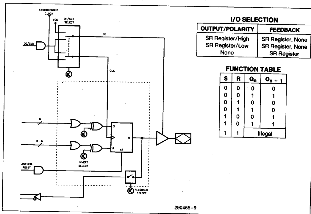
Figure 4e. SR Flip-Flop Register Configuration
