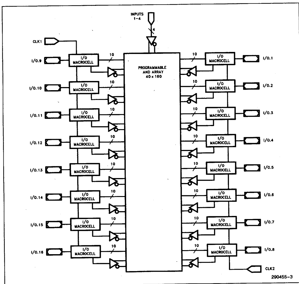
Figure 2. iPLD610 Global Architecture
