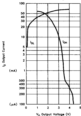
iPLD610 Output Current in Relation to Voltage
