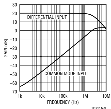
Frequency Response
