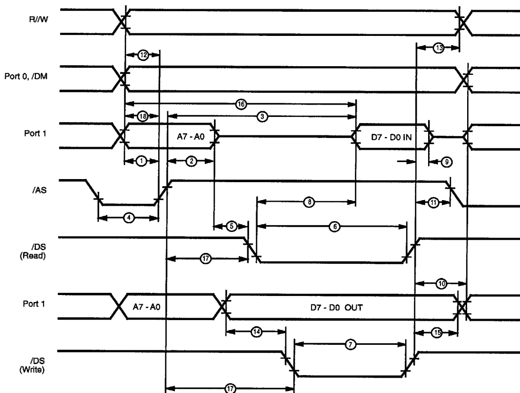
Figure 24. External I/O or Memory Read/Write Timing
