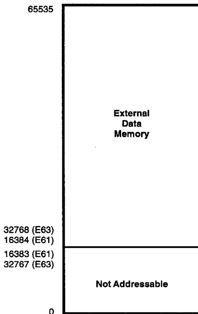
Figure 12. Data Memory Configuration
