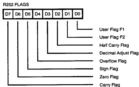
Figure 40. Flag Register (FC H : Read/Write)
