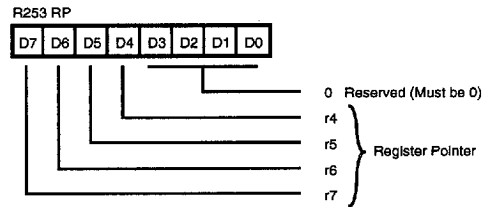
Figure 41. Register Pointer Register (FD H : Read/Write)
