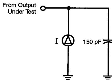
Figure 23. Test Load Diagram
