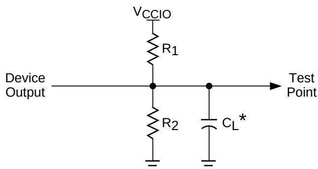
Figure 9. Test Load
