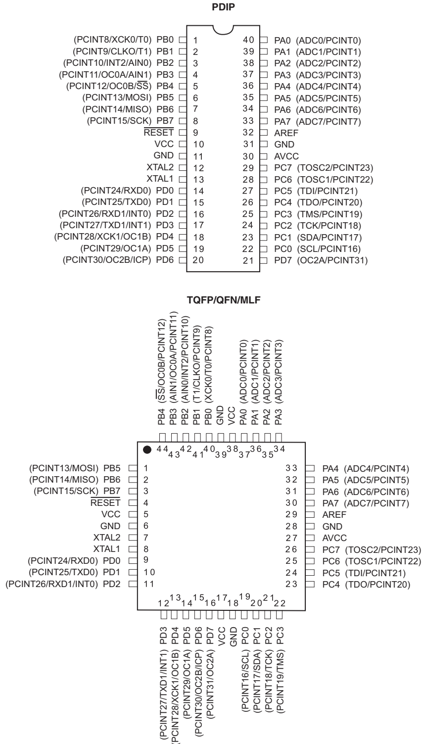
Figure 1-1. Pinout ATmega164P/324P/644P
