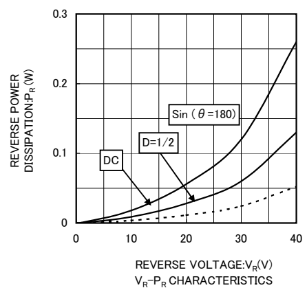
V_R - P_R CHARACTERISTICS
