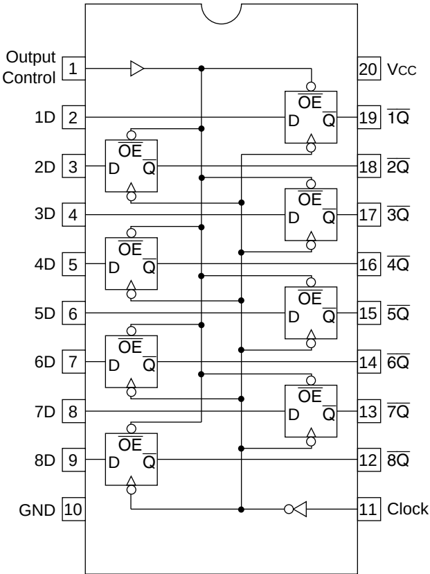
(Top view)
