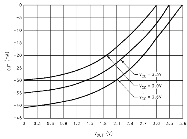
FIGURE 11. I_{OH} vs V_{OH}
