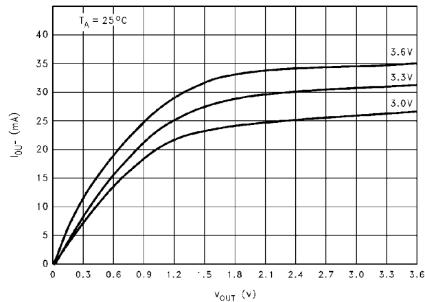
FIGURE 10. I_{OL} vs V_{OL}
