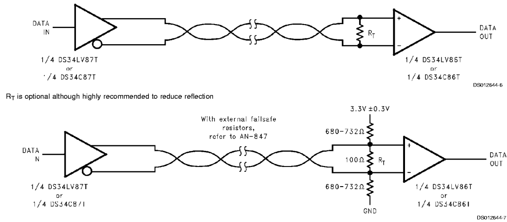
FIGURE 5. Typical Receiver Connections
