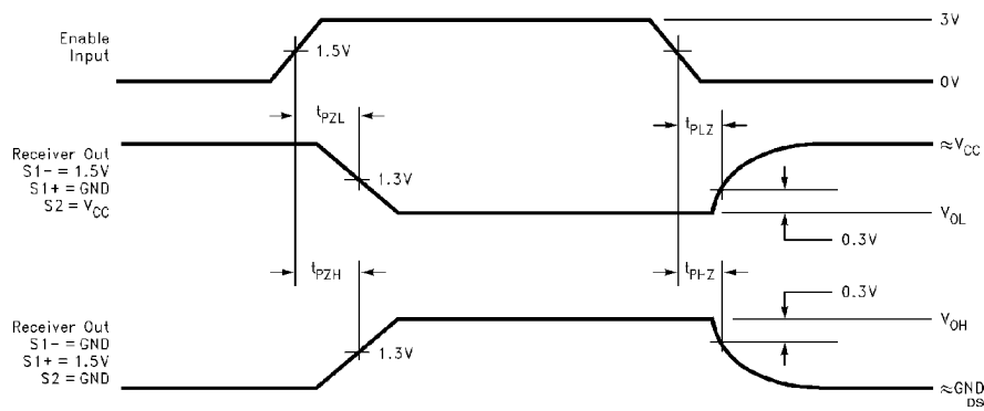
FIGURE 4. Receiver TRI-STATE Output Enable and Disable Waveforms (Note 9) (Note 10)
