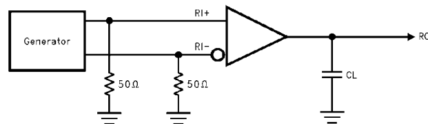
FIGURE 1. Receiver Propagation Delay and Transition Time Test Circuit (Note 9) (Note 10)
