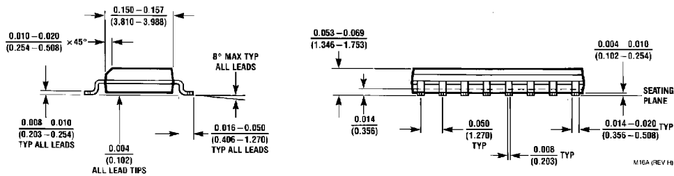
Dual-In-Line Package Order Number DS34LV86TM NS Package Number M16A
