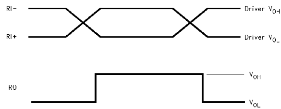
FIGURE 6. Typical Receiver Output Waveforms
