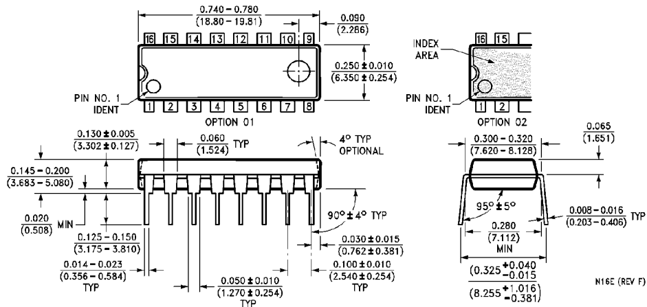
Dual-In-Line Package Order Number DS34LV86TN See NS Package Number N16E
