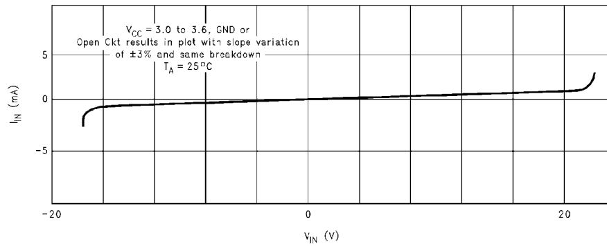
FIGURE 9. I_{IN} vs V_{IN} (Power On, Power Off)
