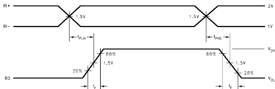
FIGURE 2. Receiver Propagation Delay and Transition Time Waveform (Note 9) (Note 10)
