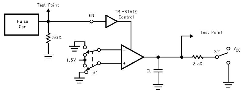
FIGURE 3. Receiver TRI-STATE Test Circuit
