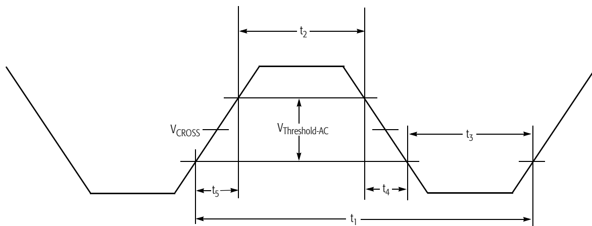
Figure 8. SYSCLK Waveform
