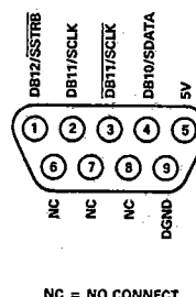
Figure 23. SKT5 Pinout
