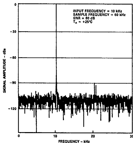
Figure 13. AD7871/AD7872 FFT Plot
