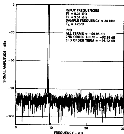
Figure 16. AD7871/AD7872 IMD Plot
