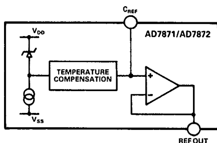
Figure 3. AD7871/AD7872 Reference Circuit
