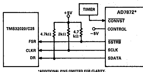
Figure 20. AD7872 to TMS32020/C25 Interface
