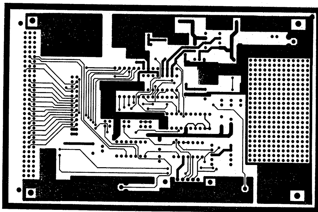
Figure 27. PCB Solder Side Layout for Figure 24
