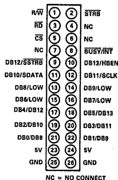
Figure 22. SKT4 Pinout
