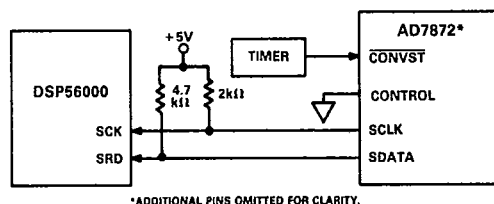
Figure 19. AD7872 to DSP56000 Interface
