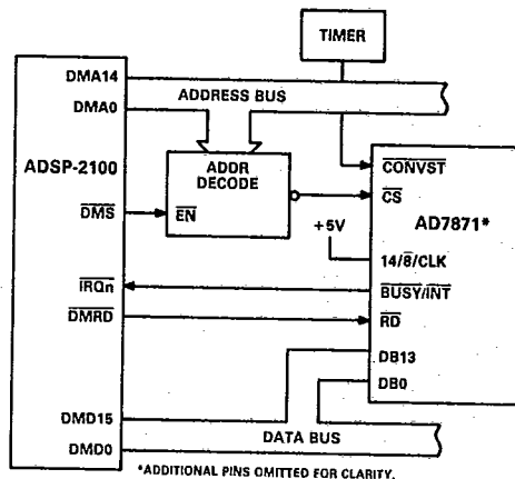
Figure 17. AD7871 to ADSP-2100 Parallel Interface
