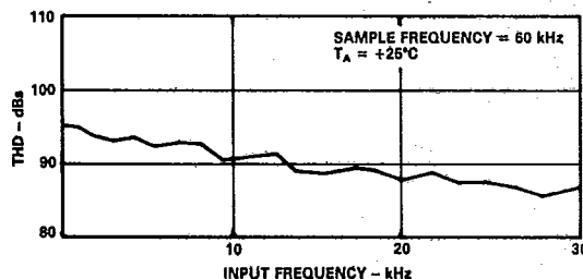
Figure 15. Total Harmonic Distortion vs. Frequency
