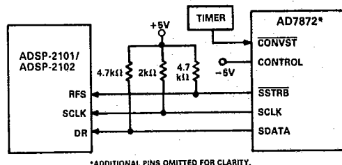
Figure 21. AD7872 to ADSP-2101/ADSP-2101 Serial Interface
