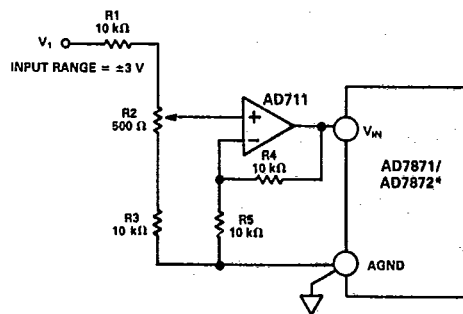
Figure 6. Bipolar Adjust Circuit
