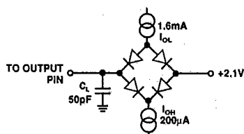
Figure 1. Load Circuit for Access Time
