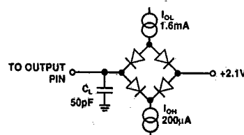
Figure 2. Load Circuit for Output Float Delay
