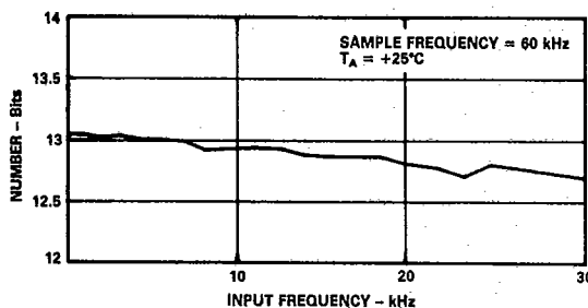
Figure 14. Effective Number of Bits vs. Frequency
