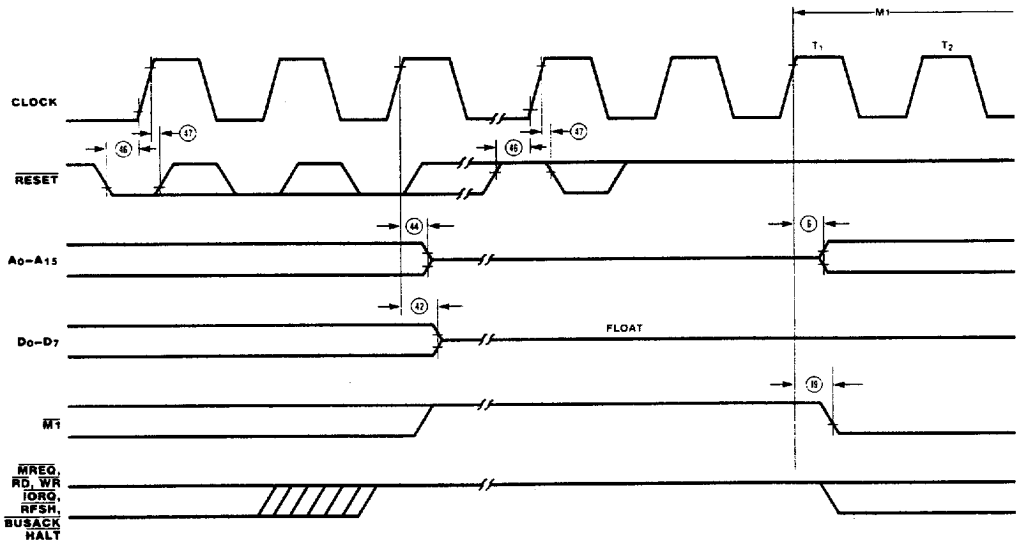
Figure 12. Reset Cycle
