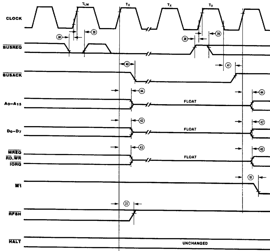
Figure 10. BUS Request/Acknowledge Cycle
