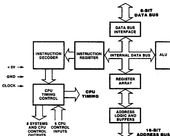
Figure 3. Z80C CPU Block Diagram
