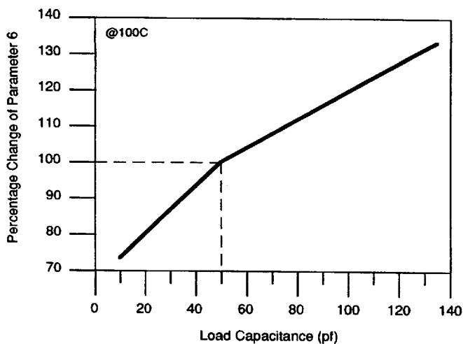
Figure 1. Address Delay Characteristics (Parameter 6)
