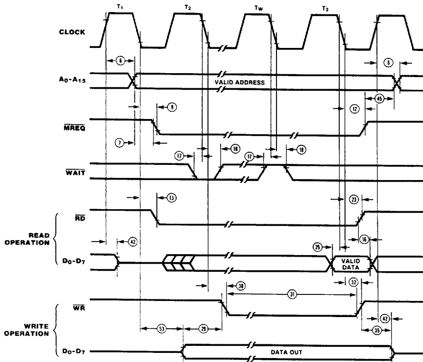
Figure 6. Memory Read or Write Cycles
