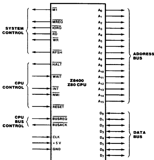
Figure 1. Pin Functions
