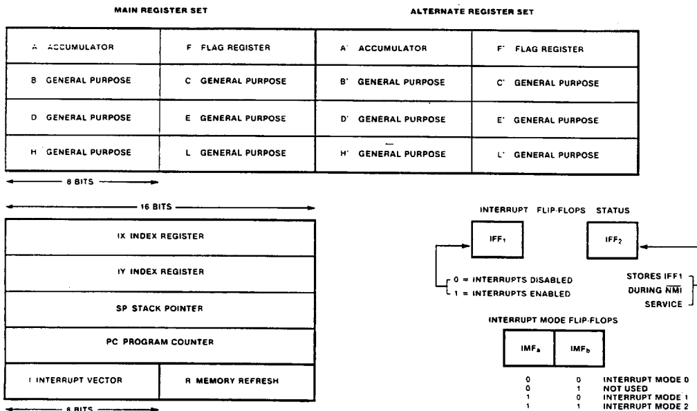
Figure 4. CPU Registers
