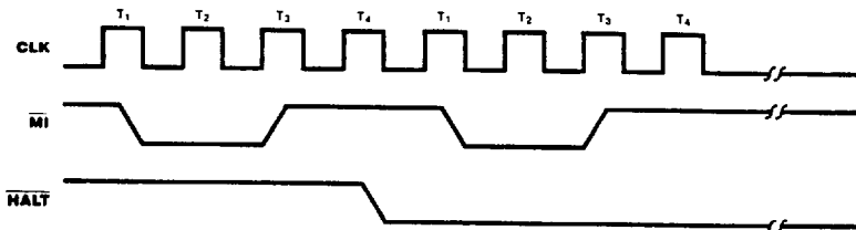
Figure 13. Power-Down Acknowledge
