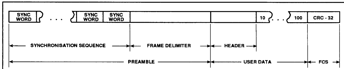
Fig 3 Generic data burst/packet format
