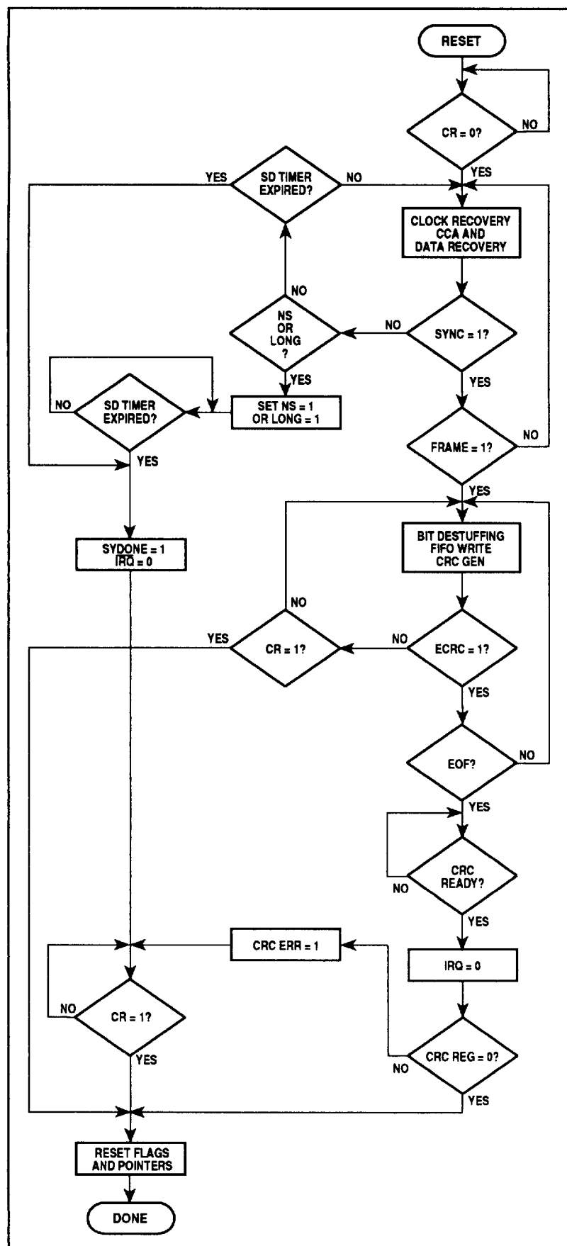
Fig. 12 Channel sense and data receive
