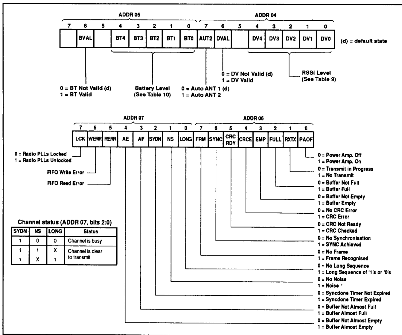
Fig. 6 Status registers (read only)
