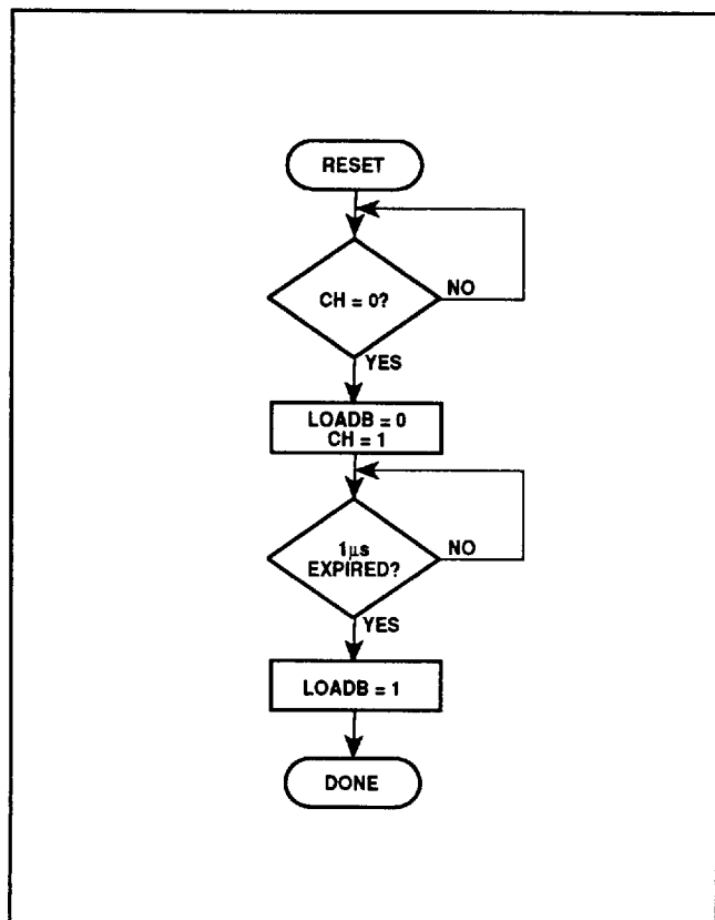
Fig. 10 Channel selection
