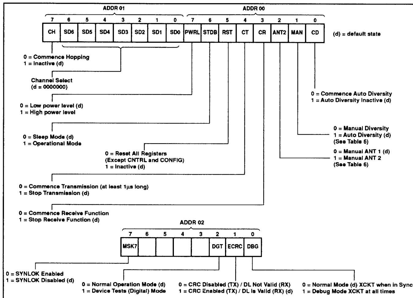
Fig. 5 Control registers (write only)
