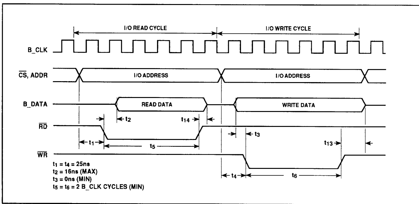
Fig. 15 Typical controller bus timing
