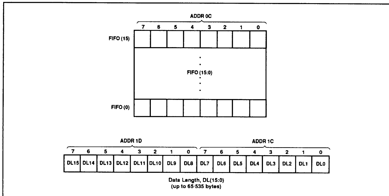
Fig. 7 Data register (FIFO) and data length registers (read/write)
