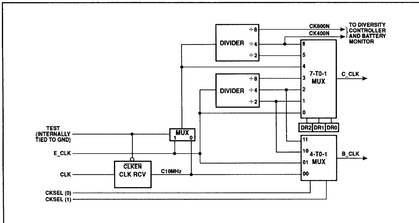
Fig. 14 Clock selector/generator
