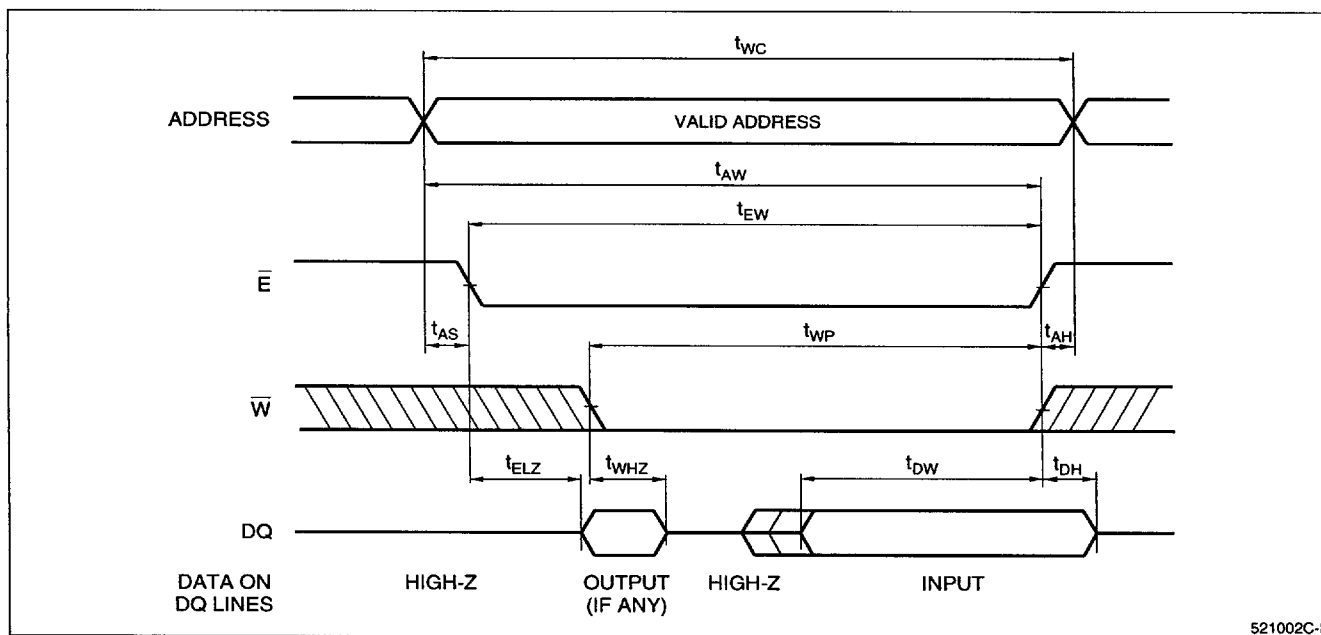
Figure 7. Write Cycle No. 2
