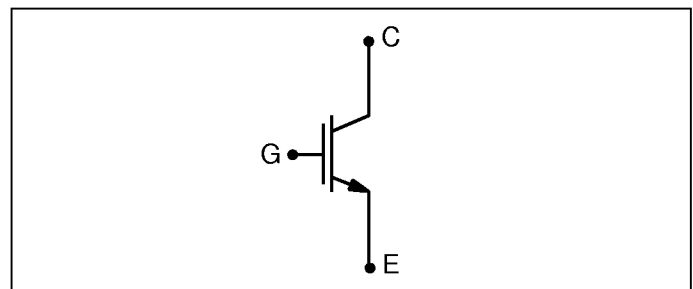
Fig.2 ITZ08F12 circuit
