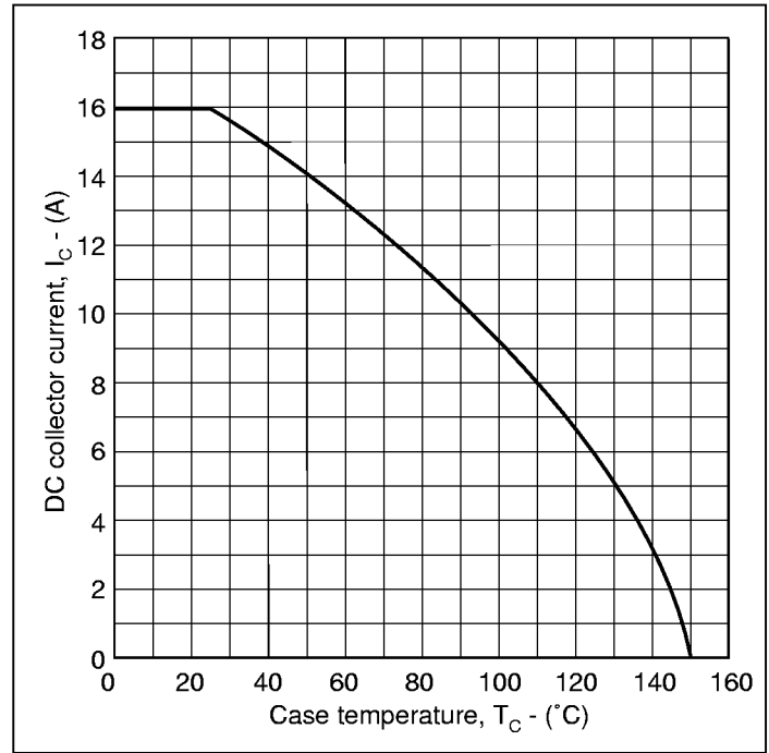
Fig.19 DC current rating vs case temperature
