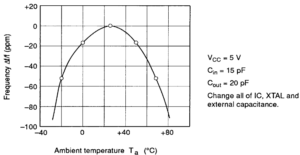
Figure 26 Frequency vs. Ambient Temperature
