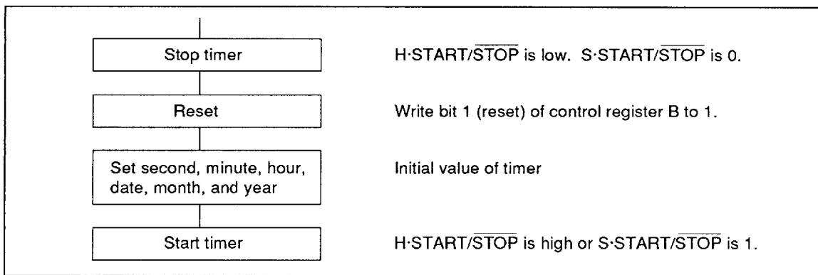
Figure 5 Timer Application
