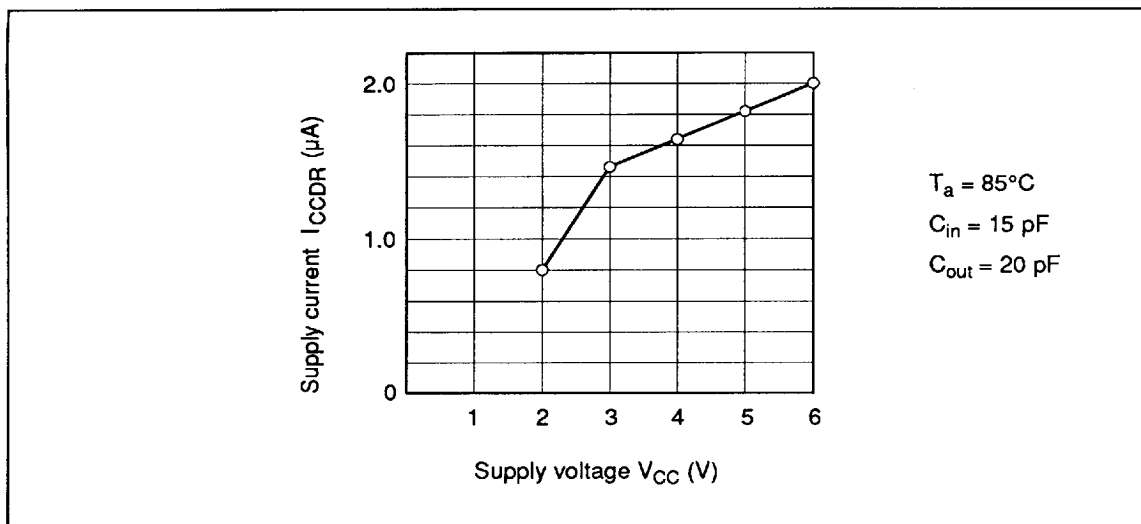
Figure 23 Supply Current vs. Supply Voltage
