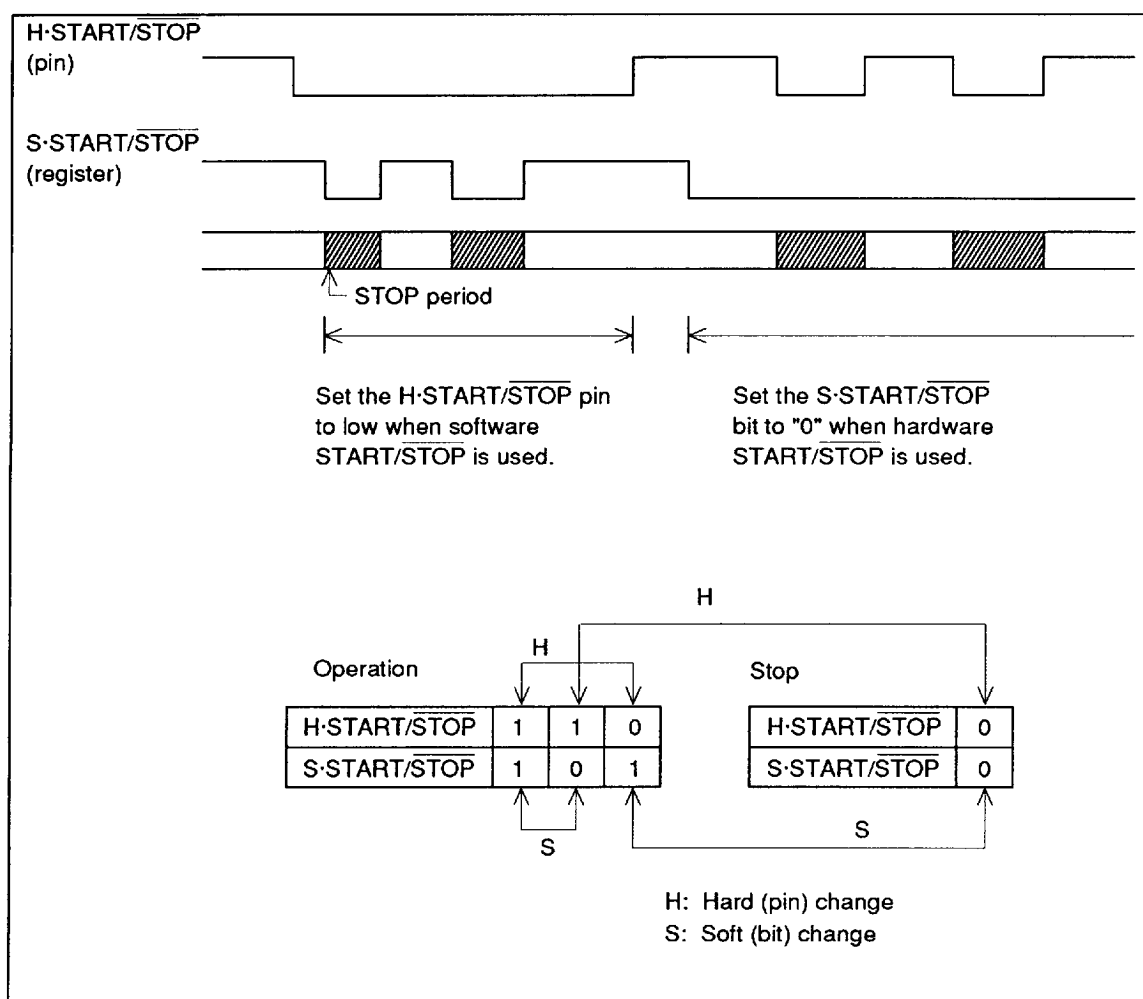
Figure 1 S-START/STOP Bit Function
