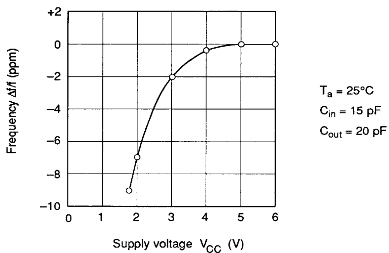
Figure 25 Frequency vs. Supply Voltage
