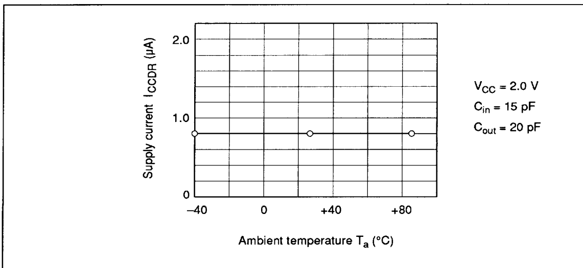
Figure 24 Supply Current vs. Ambient Temperature
