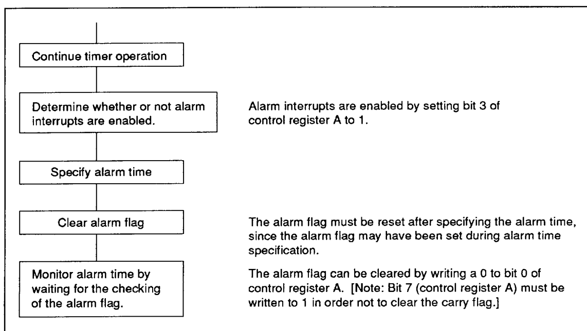
Figure 4 Alarm Function
