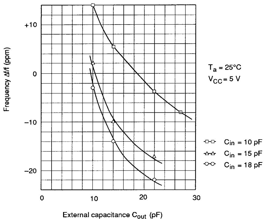
Figure 27 Frequency vs. External Capacitance
