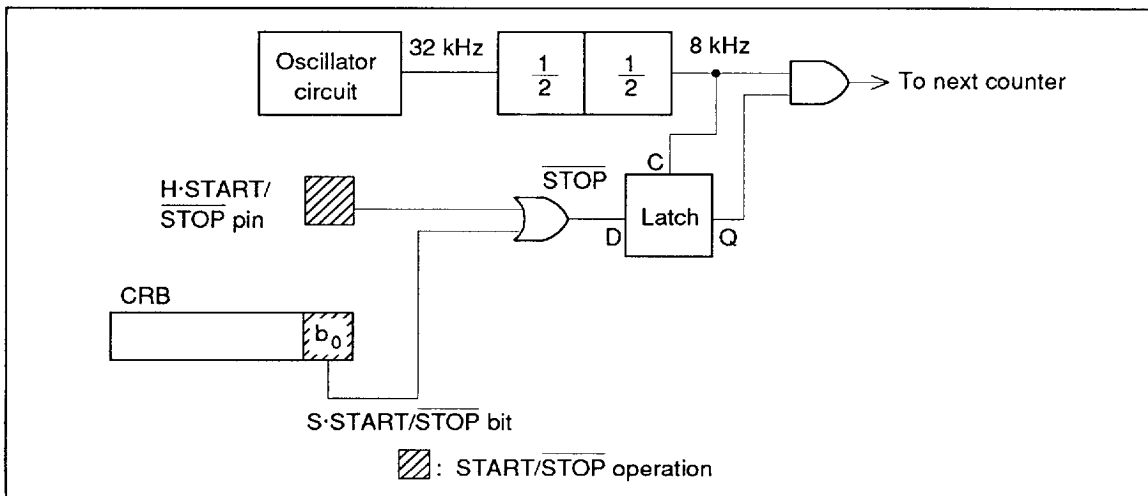
Figure 6 START/STOP Operation
