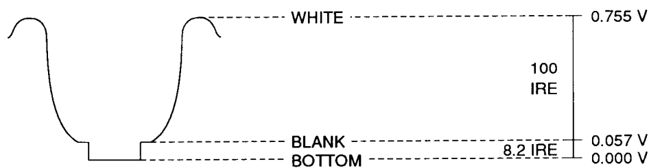
Non-composite sync, composite blanking (Red, Green, and Blue)
