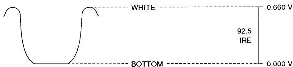
Composite sync, non-composite blanking (Green only)
