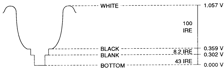
Composite sync and blanking (Green only)
