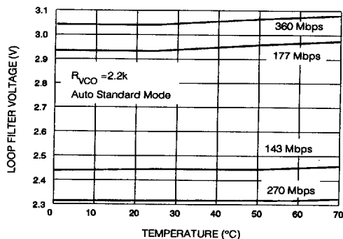
Fig. 8 Loop Filter Voltage vs Temperature
