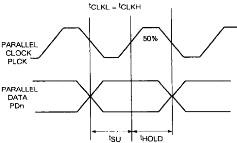
Fig. 4 Input Clock / Data Timing
