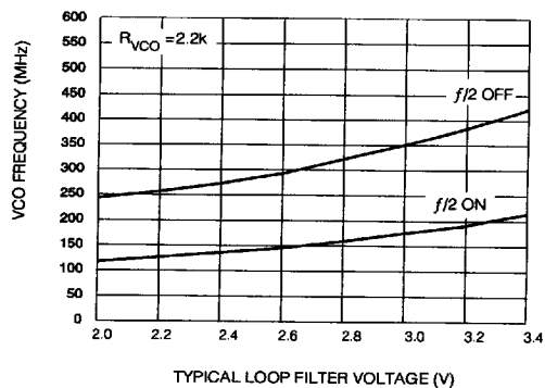
Fig. 7 VCO Frequency vs Loop Filter Voltage
