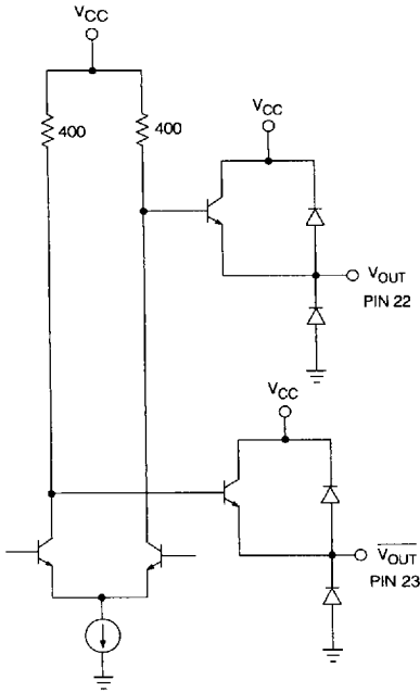
Fig. 3 Output Circuit
