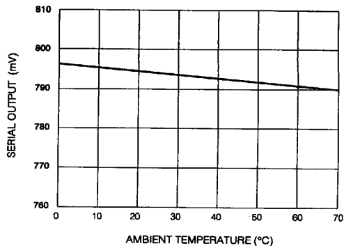
Fig. 6 Serial Data Output Level vs Temperature
