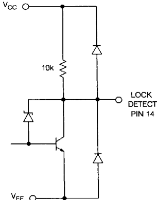
Fig. 2 Lock Detect
