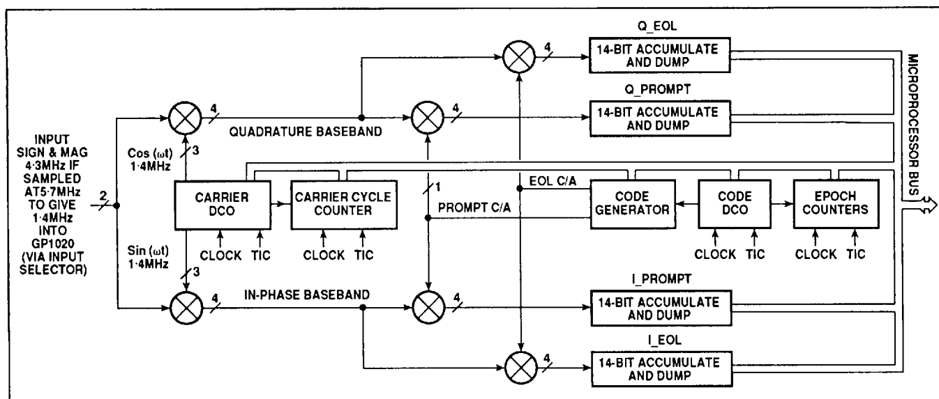
Fig. 5 Tracking module simplified block diagram
