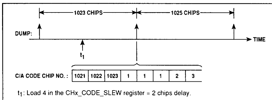
Fig. 8 SLEW in UPDATE mode
