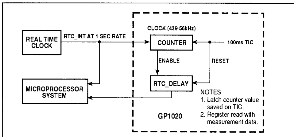
Fig. 11 RTC block diagram
