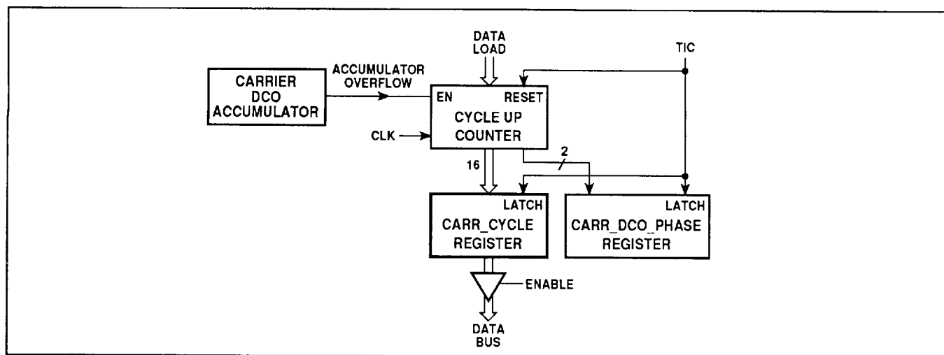
Fig. 7 CHx_CARR_CYCLE block diagram
