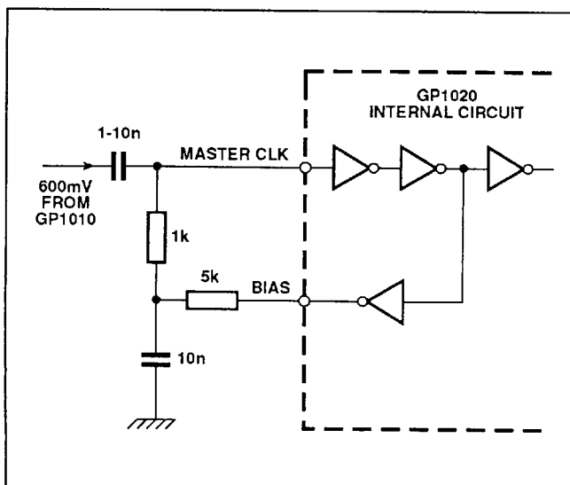
Fig. 6 Biasing circuit for master clock
