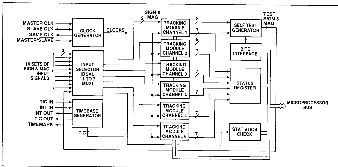
Fig. 4 Simplified overall block diagram
