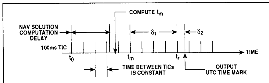
Fig. 15 TIME MARK timing diagram
