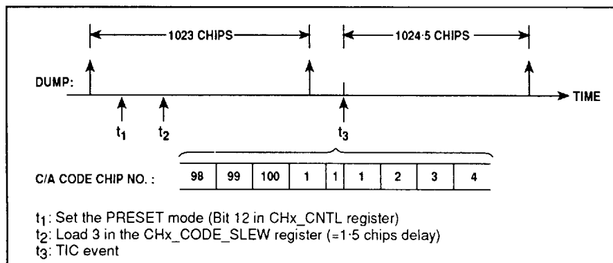
Fig. 9 SLEW in PRESET mode
