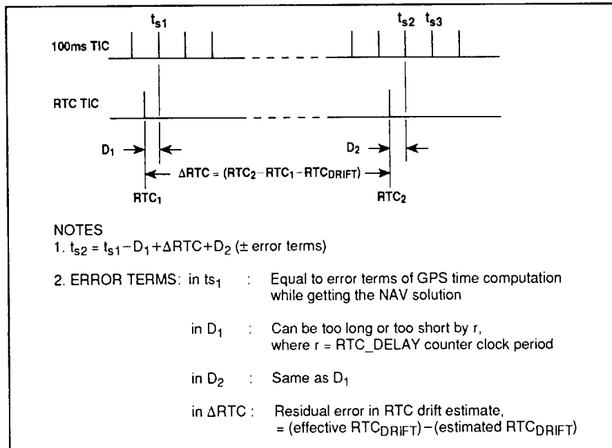
Fig. 14 Timing diagram of a short glitch
