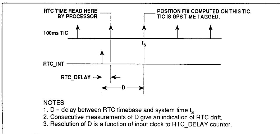
Fig. 12 RTC timing diagram
