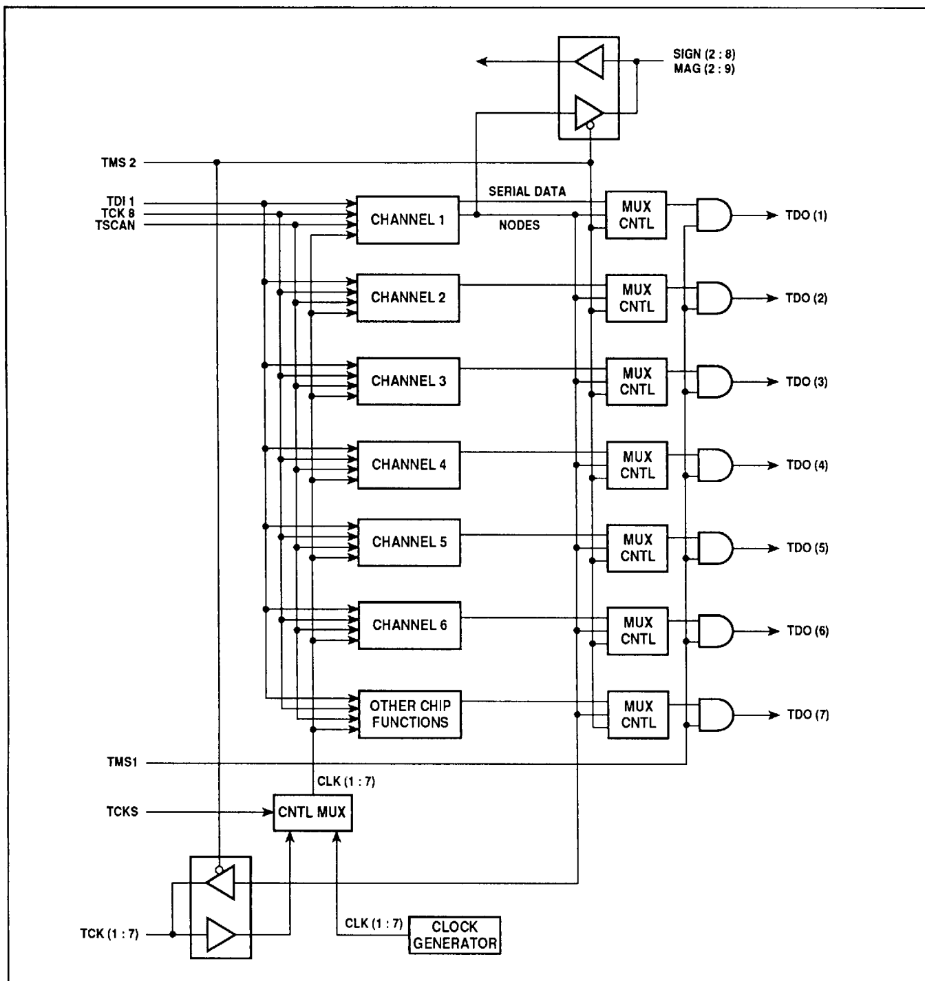
Fig. 17 Chip test functions
