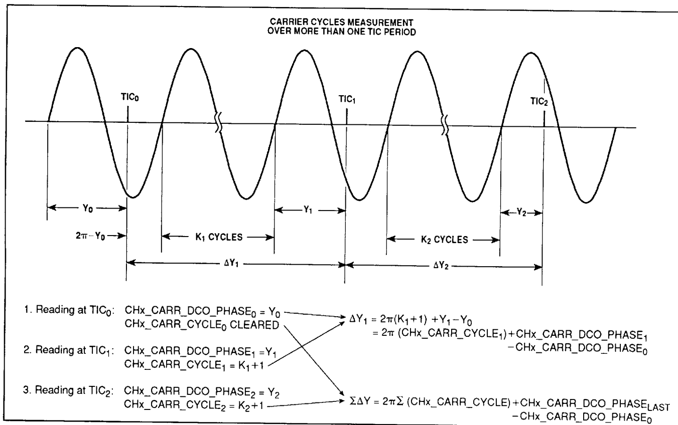
Fig. 16 Integrated carrier phase measurement
