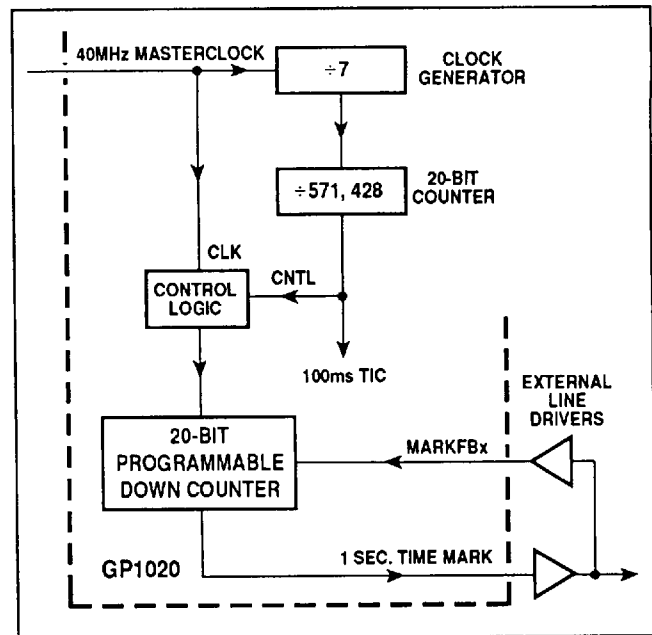
Fig. 13 Block diagram of TIME MARK generator
