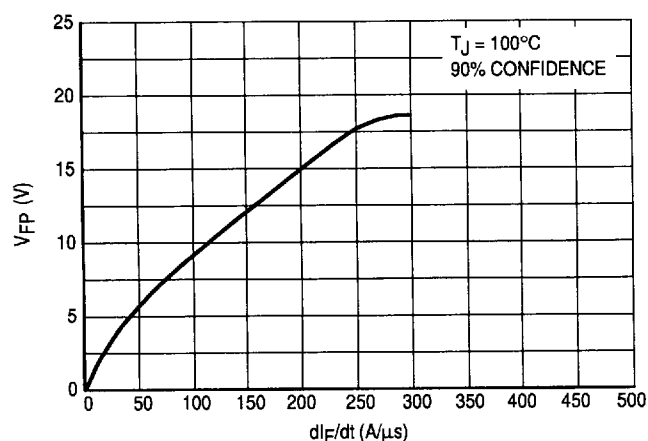
Figure 9. Peak Forward Voltage versus di/dt
