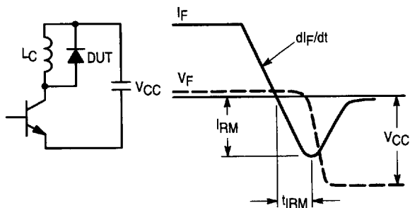
Figure 11. Turn-Off Switching Characteristics (Without series inductance)
