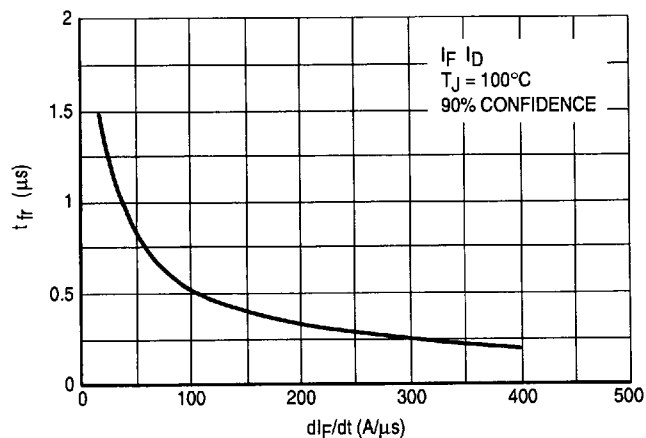
Figure 7. Recovery Time versus di/dt
