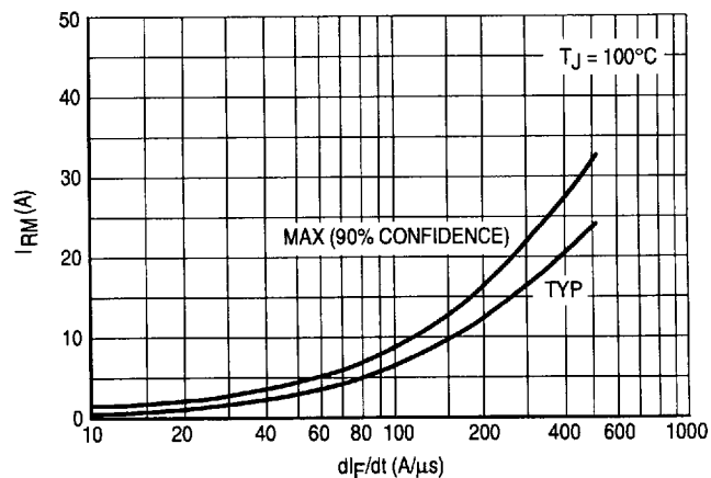
Figure 8. Peak Reverse Current versus di/dt
