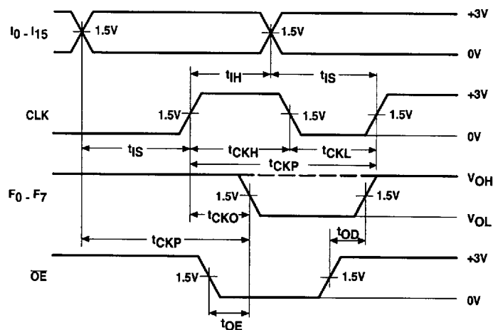
Sequential Mode
