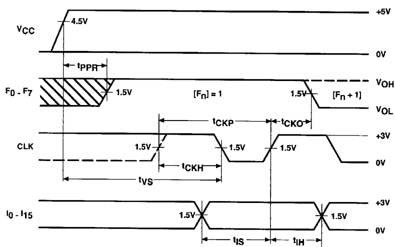
Power-On Preset
