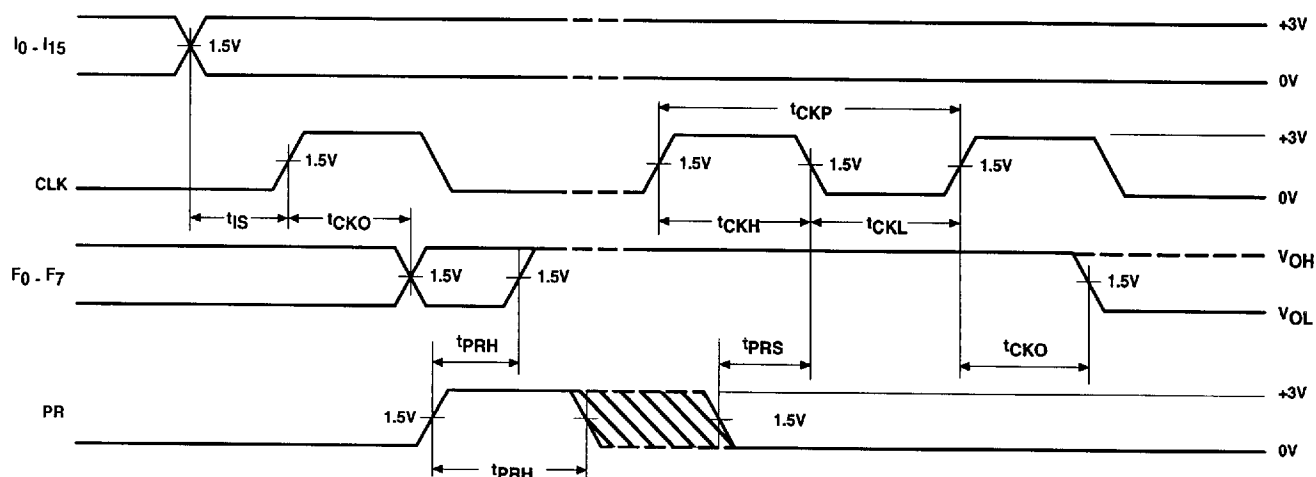
Asynchronous Preset
