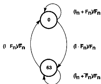
State Diagram
